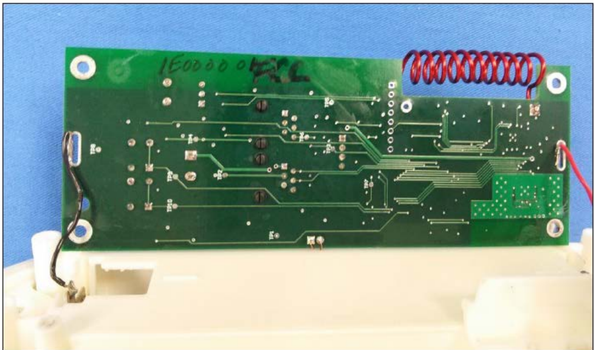
Figure 2: Rear View
