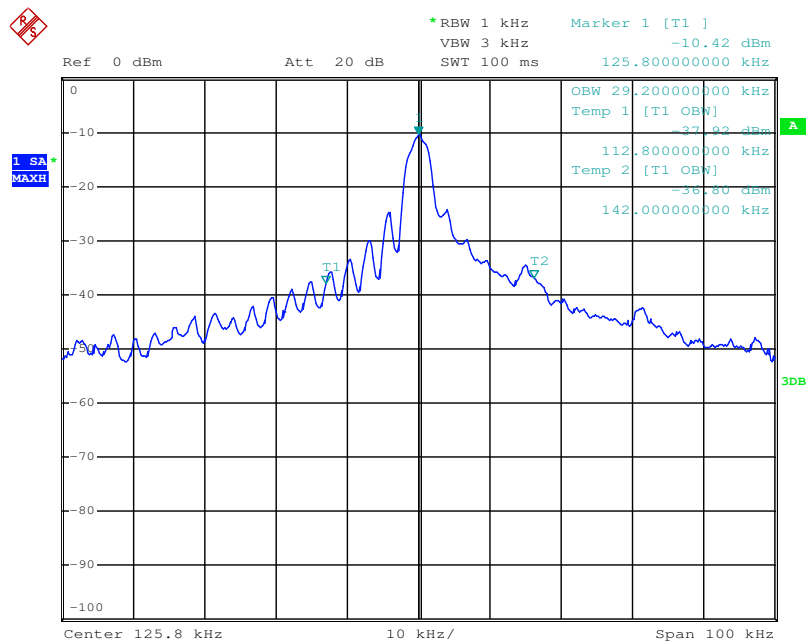
Figure 7.2.2-1: 20dB BW
