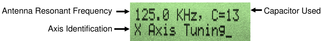
Figure 16 – Display in Tool Info Mode (Second Screen), System B
