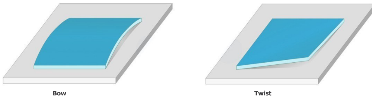
FIGURE 8-1. EXAMPLE OF BOW AND TWIST
