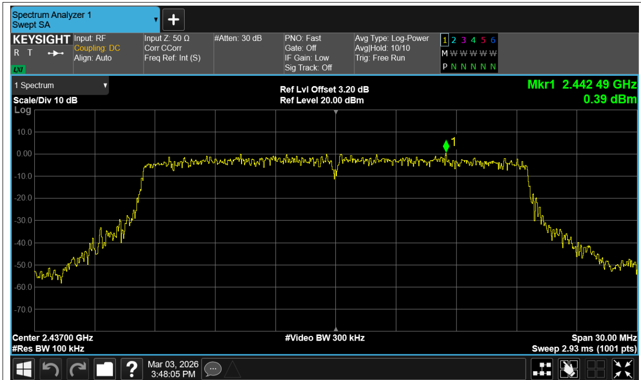
Tx. Spurious NVNT ax20 2437MHz Ant3 Emission
