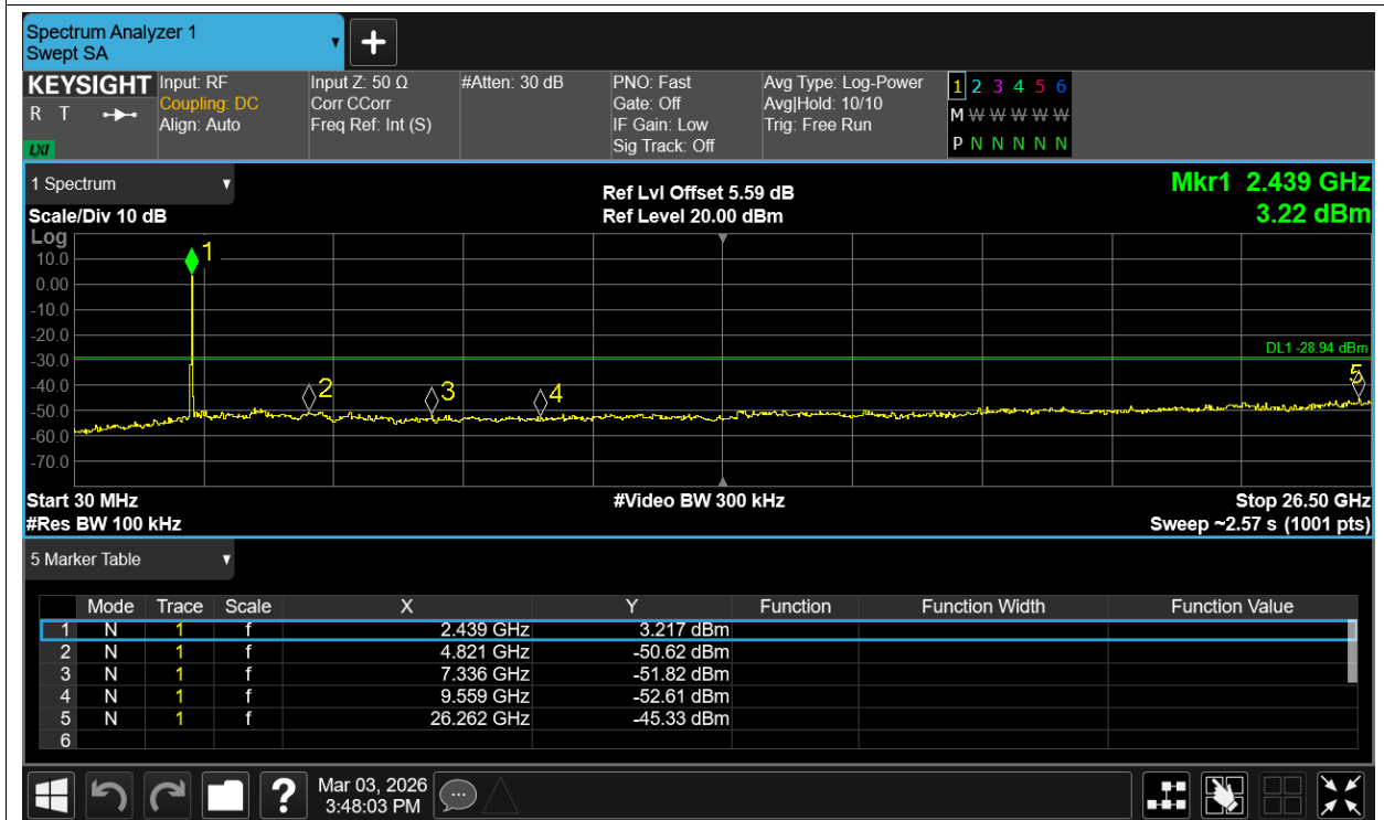
Tx. Spurious NVNT ax20 2437MHz Ant3 Ref
