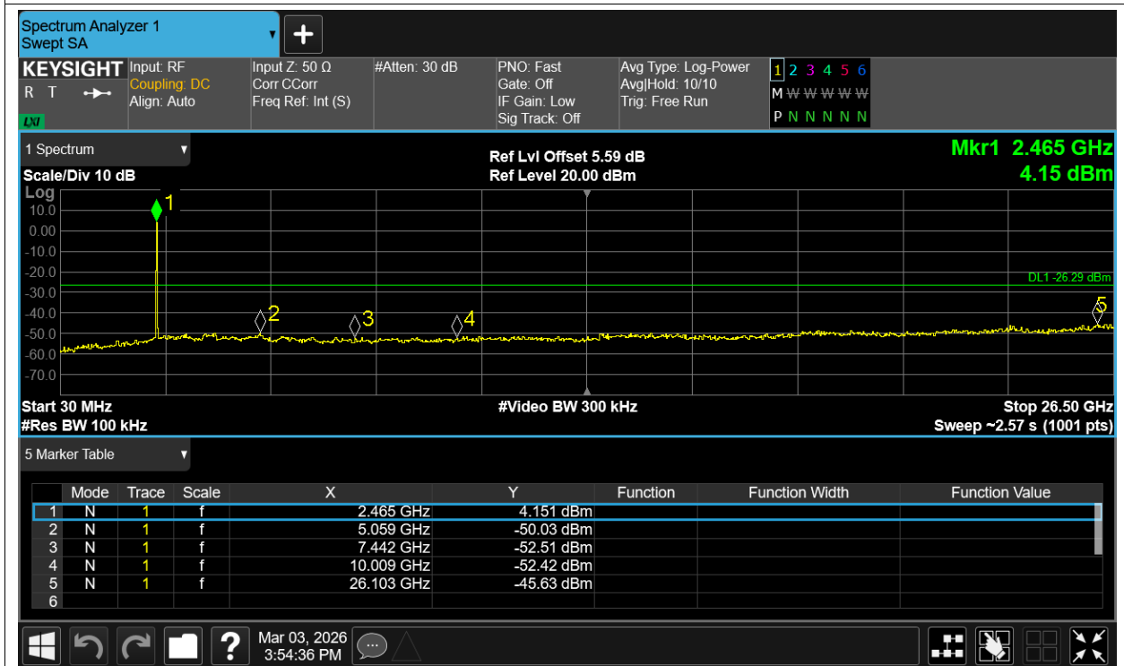
Tx. Spurious NVNT ax20 2462MHz Ant3 Ref
