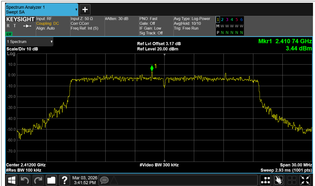
Tx. Spurious NVNT ax20 2412MHz Ant3 Emission
