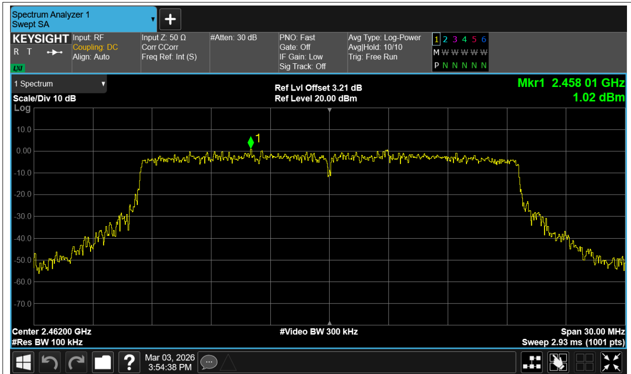
Tx. Spurious NVNT ax20 2462MHz Ant3 Emission
