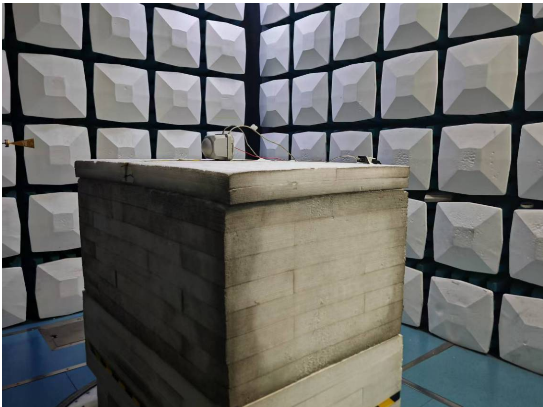
Radiated Emission 40-60GHz View TNA-AK-100
