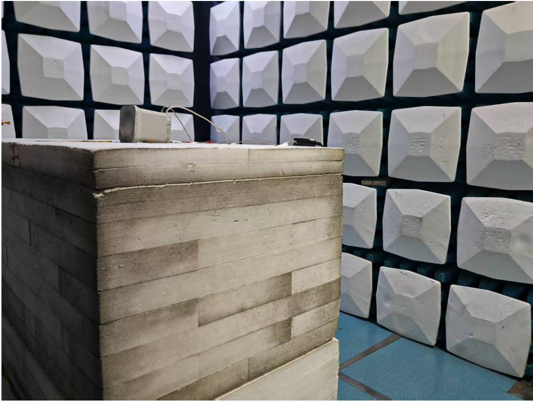
Radiated Emission 140-200GHz View TNA-AK-150
