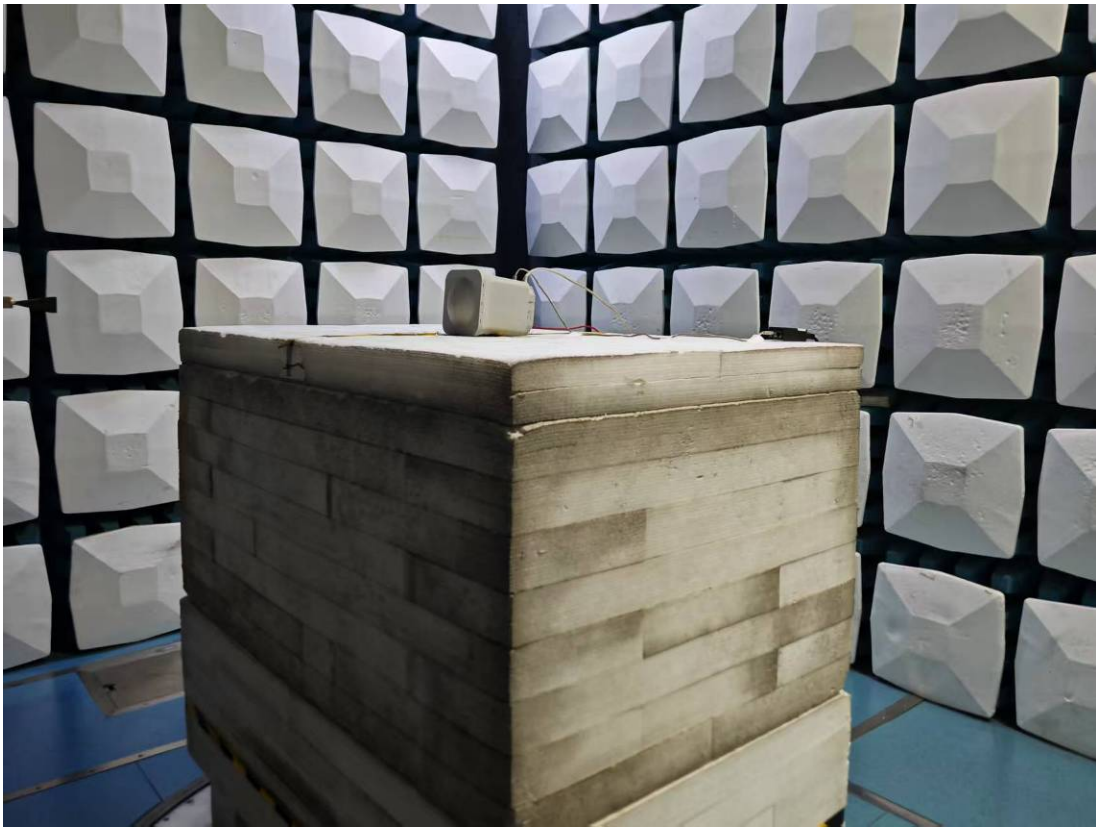
Radiated Emission 60-90GHz View TNA-AK-150
