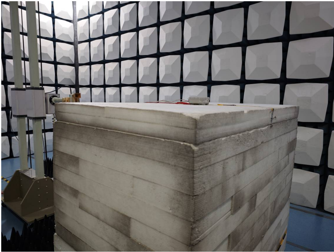
Radiated Emission 40-60GHz View Base model
