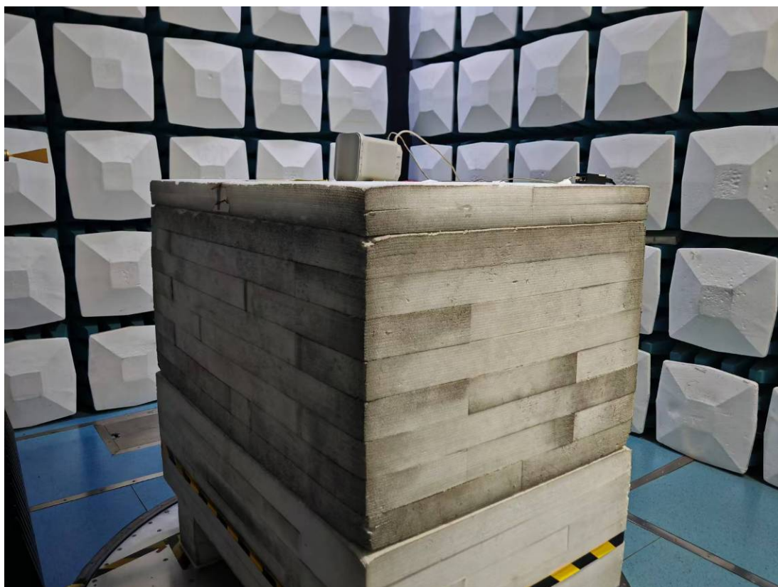
Radiated Emission 40-60GHz View TNA-AK-S-45
