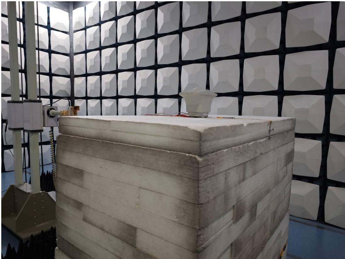
Radiated Emission 40-60GHz View TNA-AK-S-90
