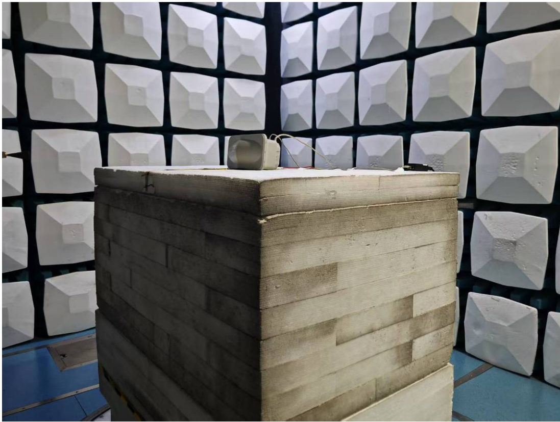
Radiated Emission 60-90GHz View TNA-AK-S-90
