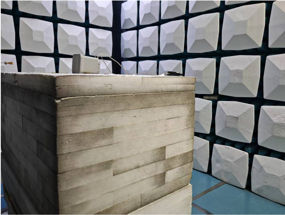
Radiated Emission 140-200GHz View TNA-AK-S-45
