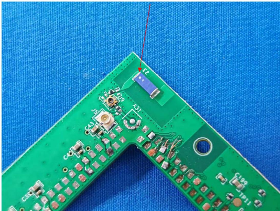
Chip Antenna Chain 1
