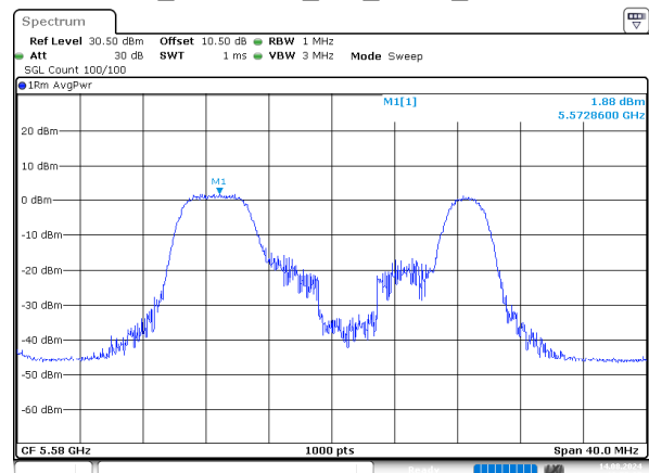
ax20_5580MHz_RU_52/37_Chain 1
