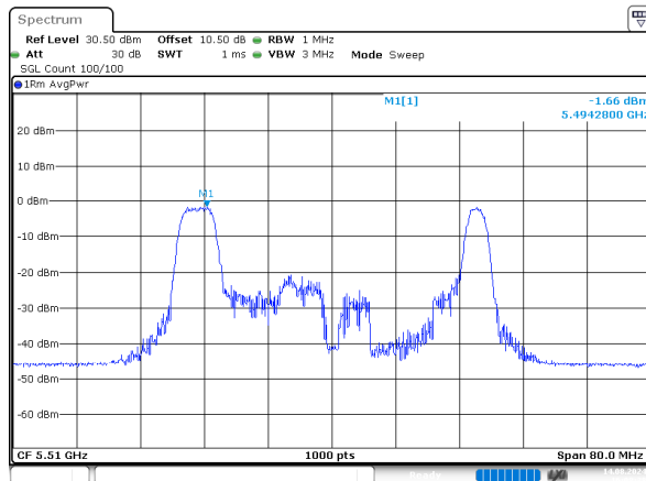
ax40_5510MHz_RU_52/37_Chain 1
