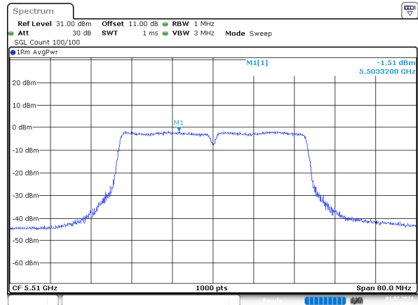
ac40_5510MHz_Chain 1
