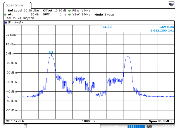
ax40_5670MHz_RU_26/17_Chain 1
