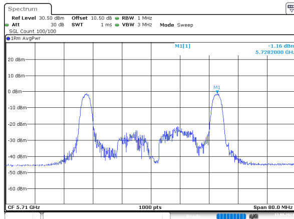
ax40_5710MHz_RU_26/17_Chain 0
