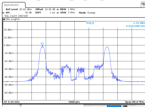
ax40_5550MHz_RU_26/0_Chain 0
