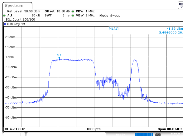
ax40_5510MHz_RU_242/61_Chain 1
