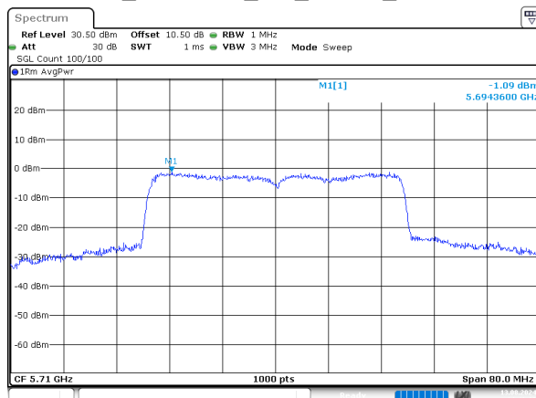
ax40_5710MHz_RU_484/65_Chain 0
