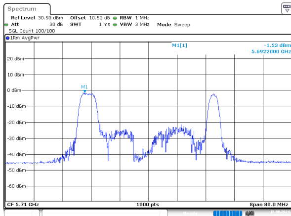
ax40_5710MHz_RU_52/44_Chain 1
