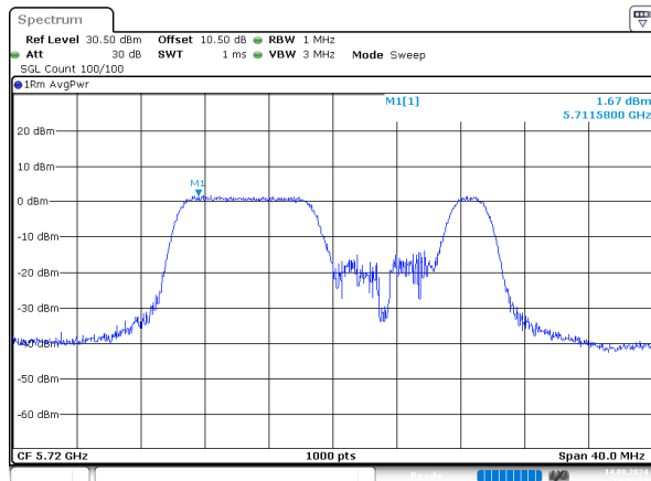
ax20_5720MHz_RU_106/54_Chain 1
