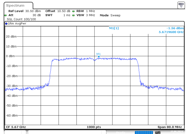
ax40_5670MHz_RU_484/65_Chain 1
