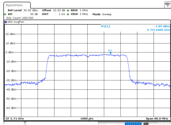
ax40_5710MHz_RU_484/65_Chain 1
