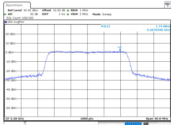
ax20_5580MHz_RU_242/61_Chain 0
