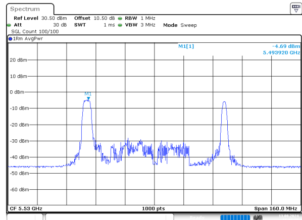
ax80_5530MHz_RU_52/37_Chain 0
