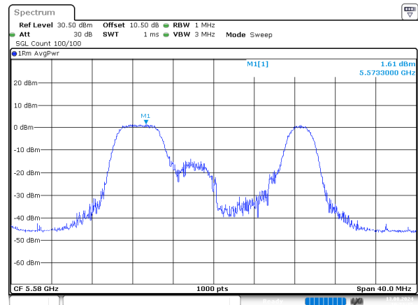
ax20_5580MHz_RU_52/37_Chain 0
