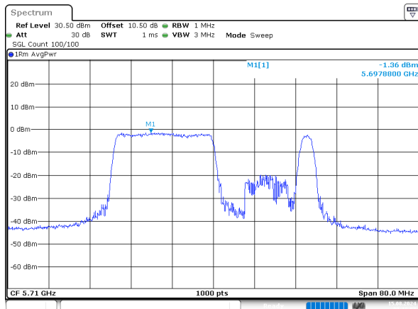
ax40_5710MHz_RU_242/62_Chain 1
