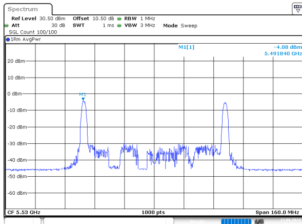
ax80_5530MHz_RU_26/0_Chain 0
