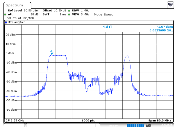
ax40_5670MHz_RU_106/56_Chain 1
