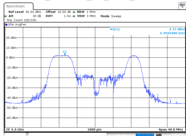
ax20_5500MHz_RU_52/37_Chain 0
