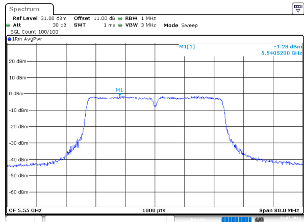
ac40_5550MHz_Chain 1
