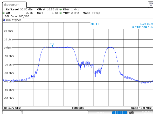
ax20_5720MHz_RU_106/54_Chain 0
