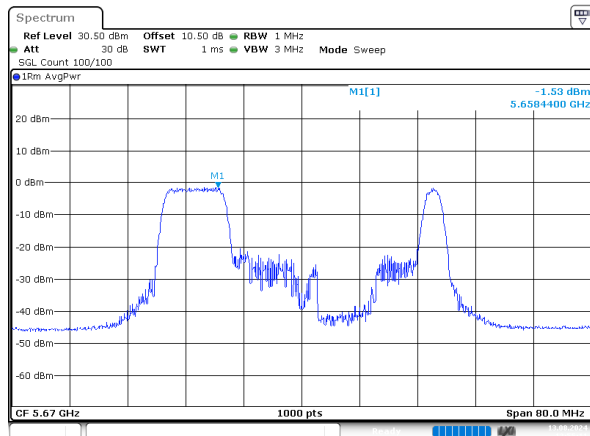
ax40_5670MHz_RU_106/56_Chain 0
