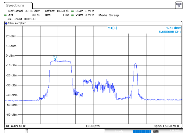
ax80_5690MHz_RU_242/64_Chain 1
