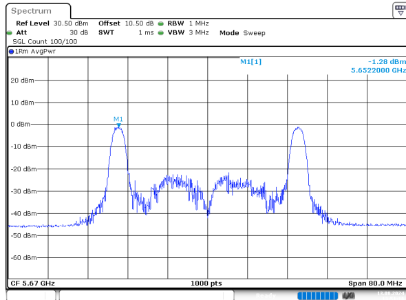
ax40_5670MHz_RU_26/17_Chain 0
