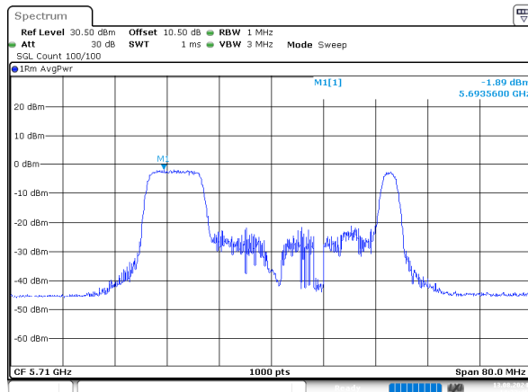
ax40_5710MHz_RU_106/56_Chain 0
