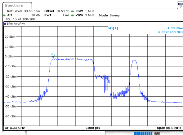
ax40_5550MHz_RU_242/61_Chain 1
