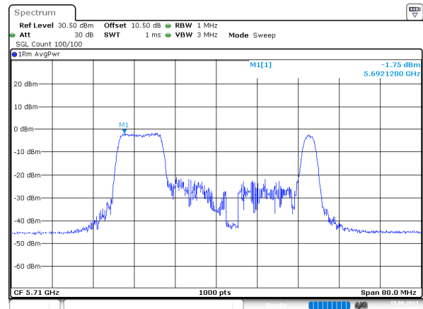
ax40_5710MHz_RU_106/56_Chain 1
