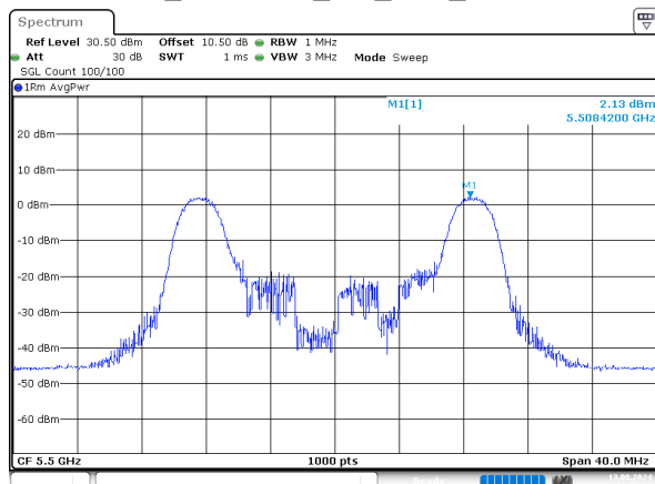
ax20_5500MHz_RU_26/0_Chain 0
