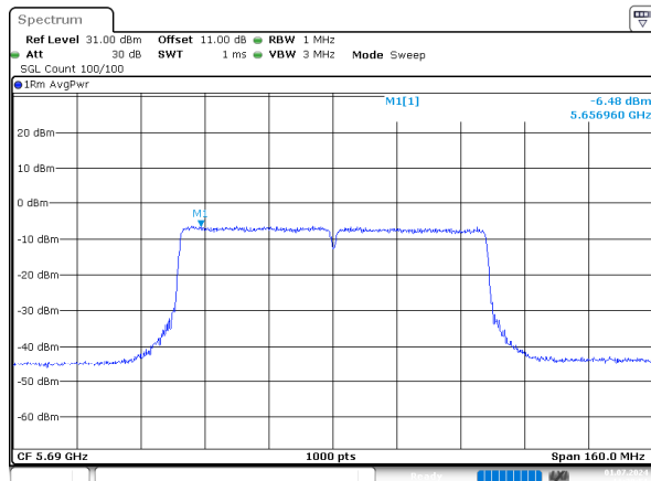
ac80_5690MHz_Chain 0
