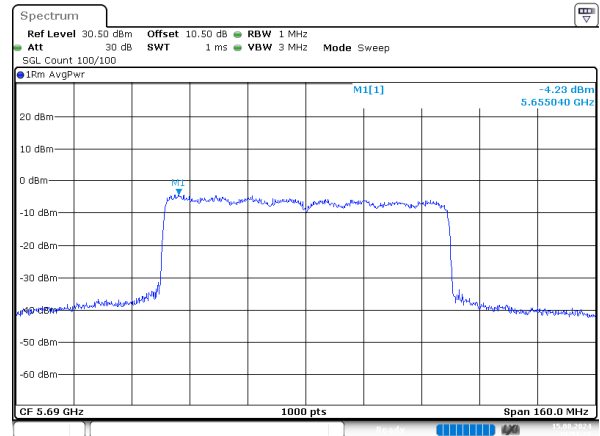
ax80_5690MHz_RU_996/67_Chain 1
