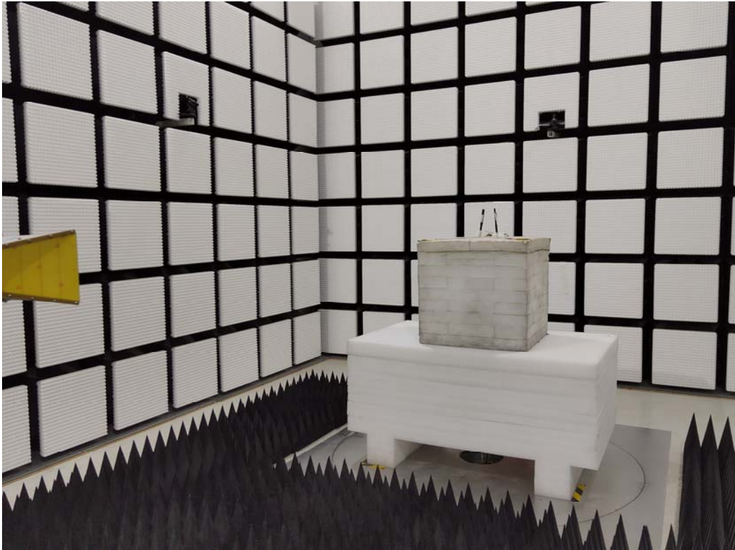
Radiated Emissions Above 1G -Whip Antenna
