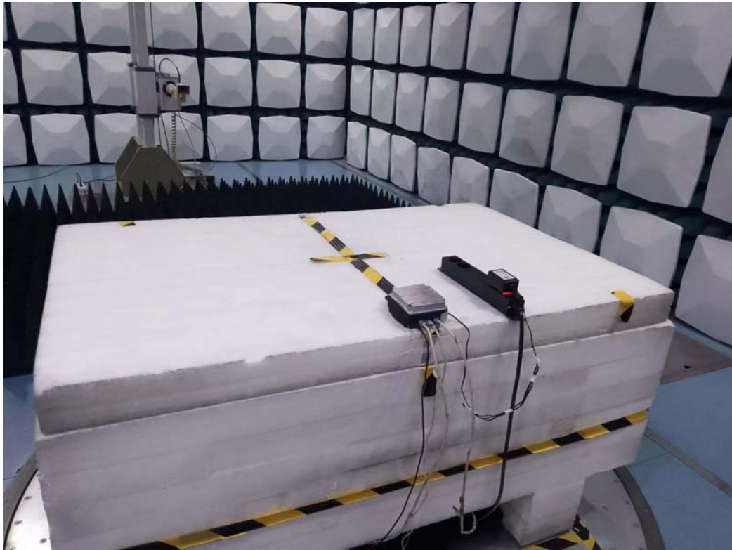
Radiated Emissions 18-26.5G View
