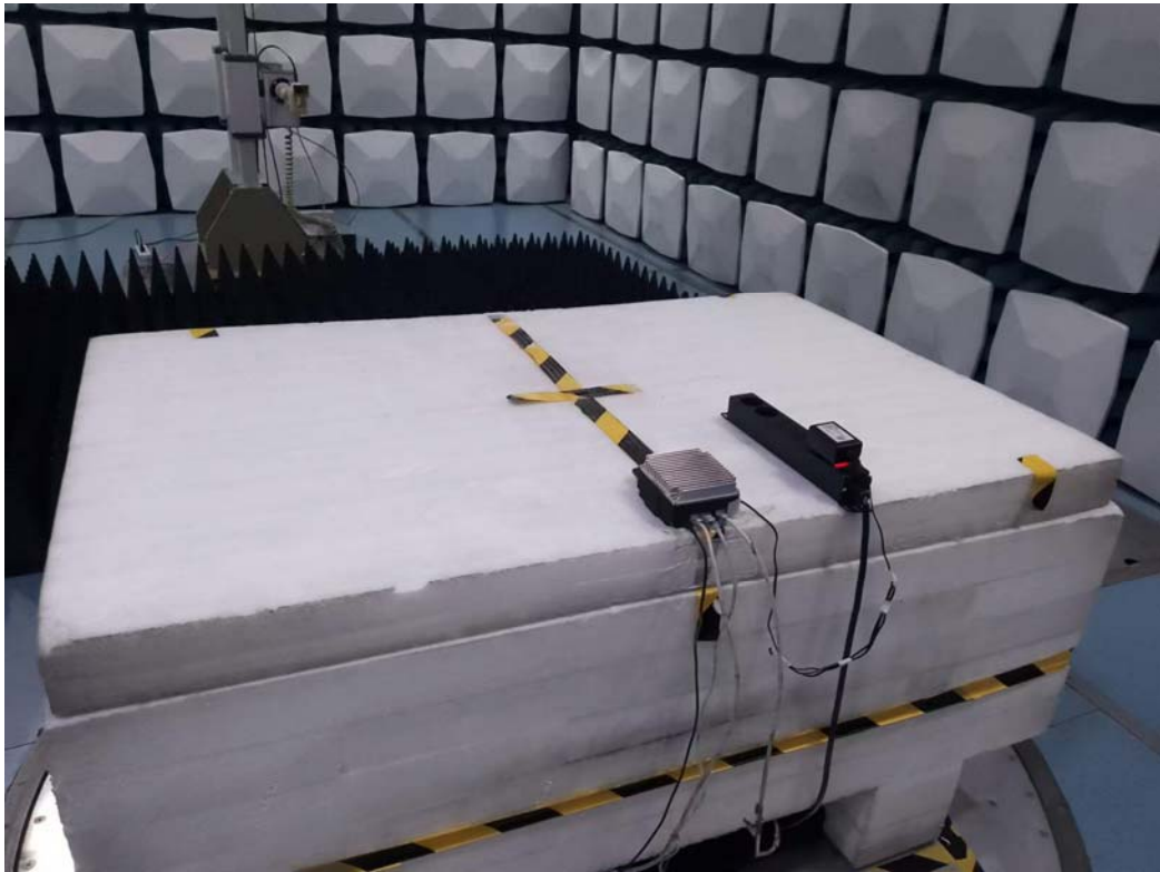
Radiated Emissions 26.5-30G View
