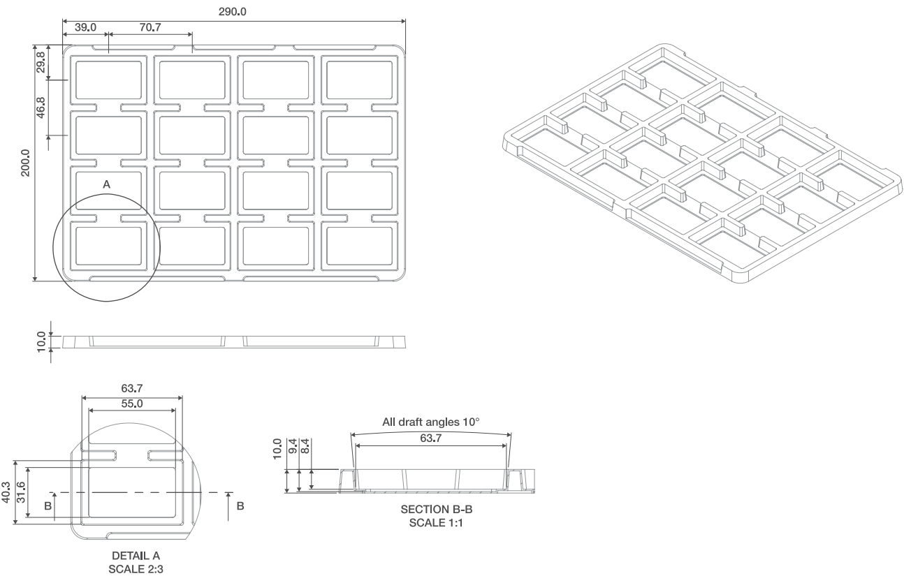
FIGURE 13-1. TRAY DIMENSIONS
