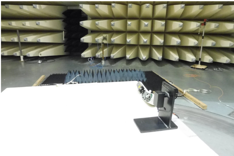
Photo 2: Radiated Emission
