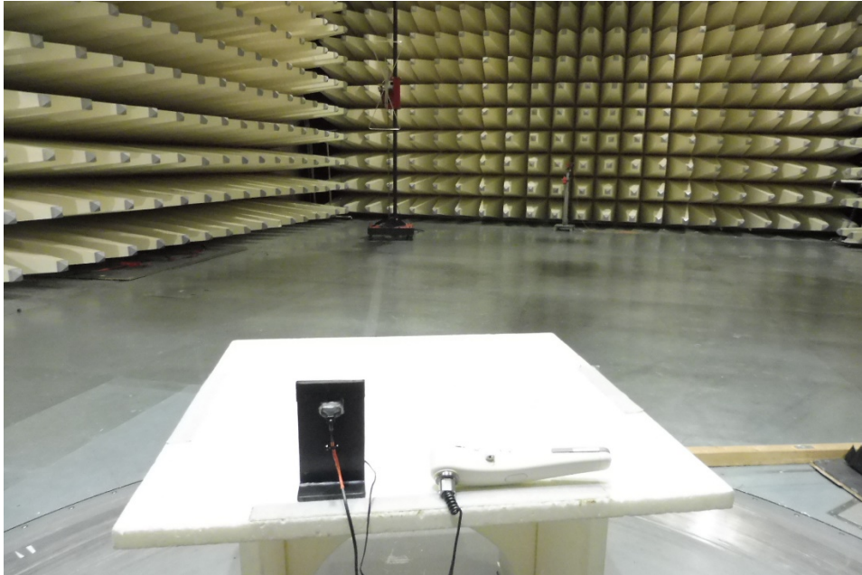
Photo 1: Radiated Emission
