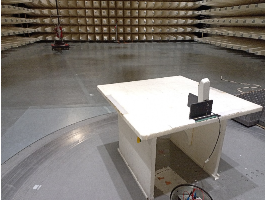
Photo 1: Radiated Emission
