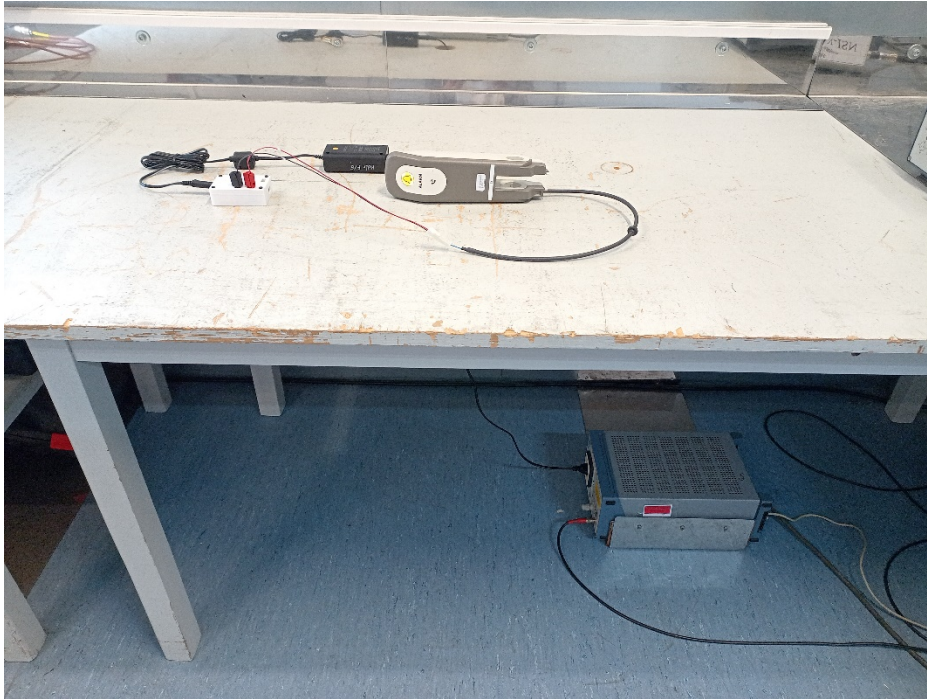
Photo 3: Conducted Emission
