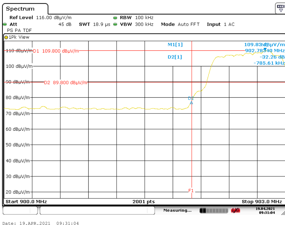
Plot 12. showing more than 20 dB band edge attenuation, EUT in Hopping mode F1 shows the band edge frequency of 902 MHz
