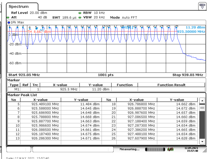
Plot: 26 channels in the range 925-928 MHz
