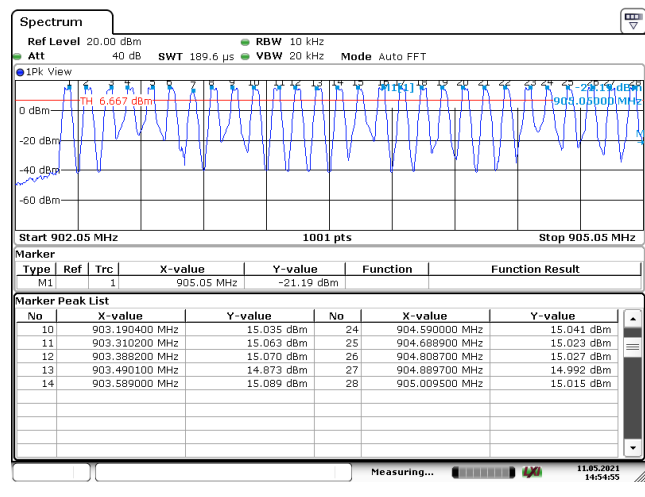
Plot: 28 channels in the range 902-905 MHz
