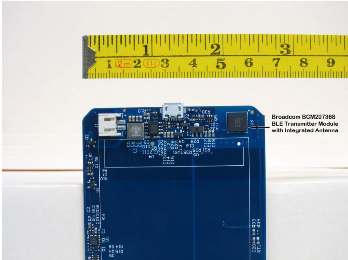
PCB detail
