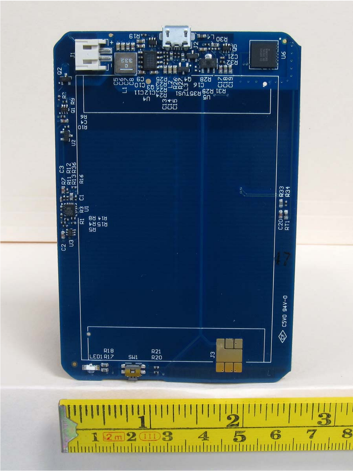
PCB Front
