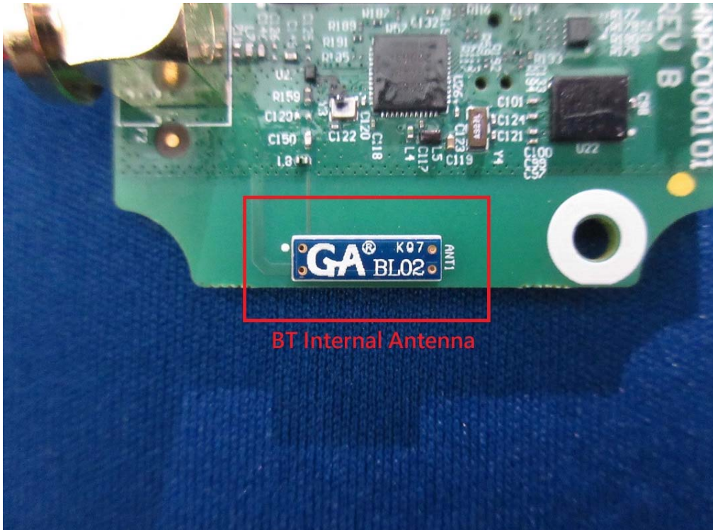
(12) EUT Photo (BT Internal Antenna)
