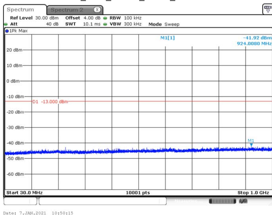
PCS_1900_CH512_GPRS_Below 1G
