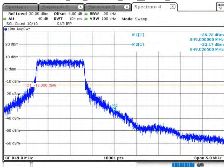
CAT-M1_B26_CH26990_10M_QPSK_6RB0
