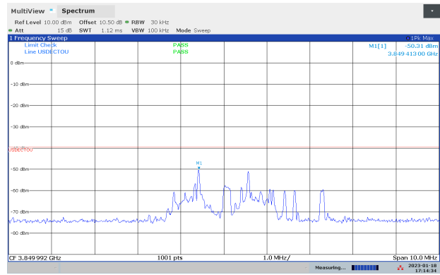
Out-of-Band Emissions, Middle Channel, 3850 MHz
