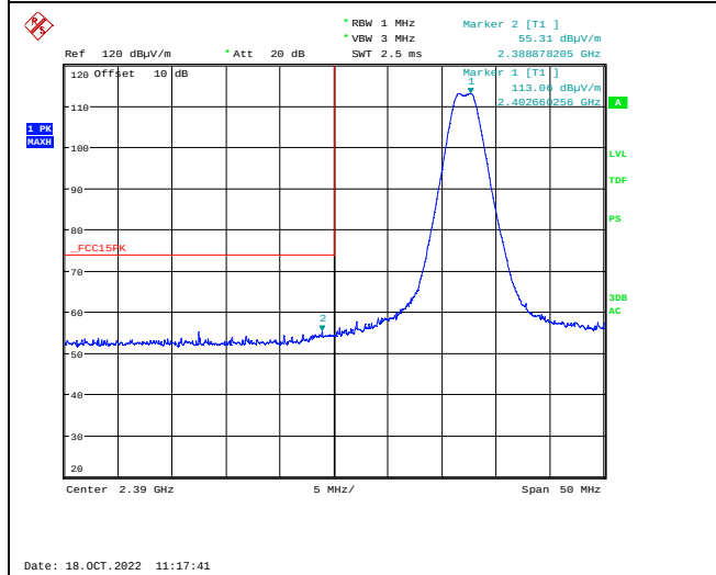
Lower Band Edge, 2402 MHz, 2Mb, Peak
