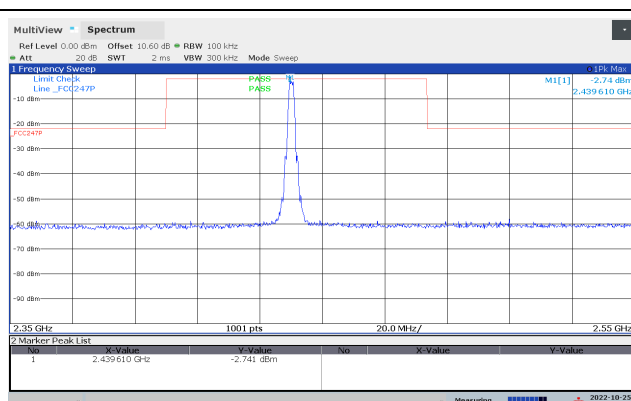
Conducted Emissions 2350-2550 MHz, 2440 MHz, 2Mb
