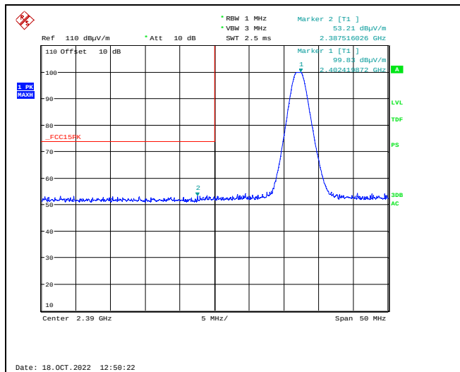
Lower Band Edge, 2402 MHz, 1Mb, Peak
