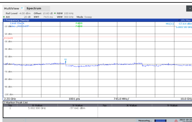
Conducted Emissions 2.55-10 GHz, 2402 MHz, 2Mb
