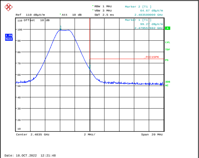
Upper Band Edge, 2480 MHz, 2Mb, Peak
