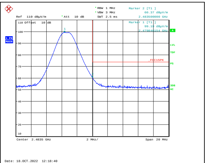
Upper Band Edge, 2480 MHz, 1Mb, Peak
