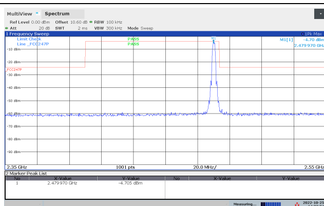
Conducted Emissions 2350-2550 MHz, 2480 MHz, 2Mb
