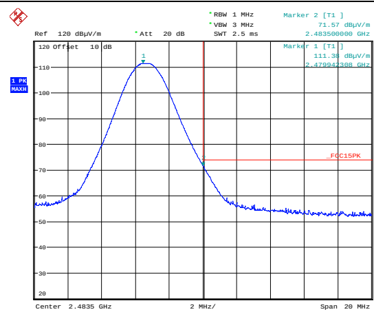
Upper Band Edge 2480 MHz, GFSK, Peak
