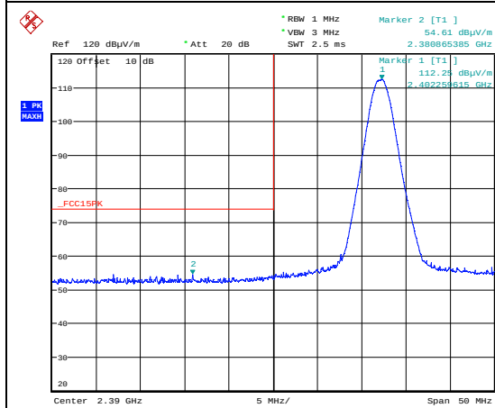
Lower Band Edge 2402 MHz, GFSK, Peak
