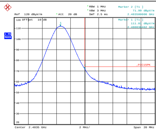
Upper Band Edge 2480 MHz, \pi/4 -DPSK, Peak
