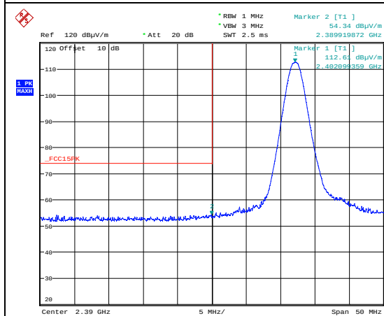
Lower Band Edge 2402 MHz, \pi/4 -DPSK, Peak
