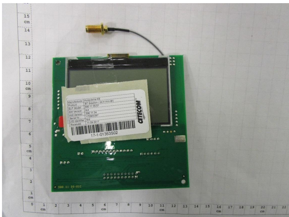
Photograph 2: EUT A Bottom side
