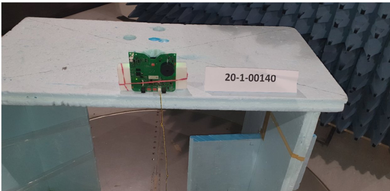
Photograph 4: EUT Setup Magnetic Field Measurements – close view
