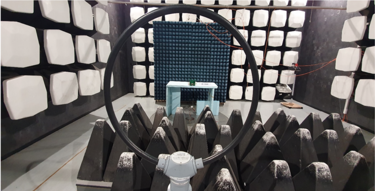
Photograph 3: EUT Setup Magnetic Field Measurements – overall view
