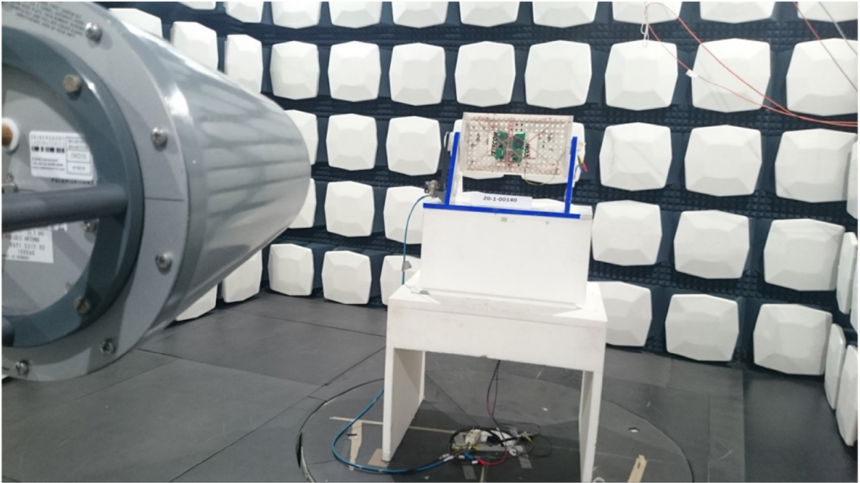
Photograph 1: EUT Test Setup, Radiated field strength above 1GHz – overall view
