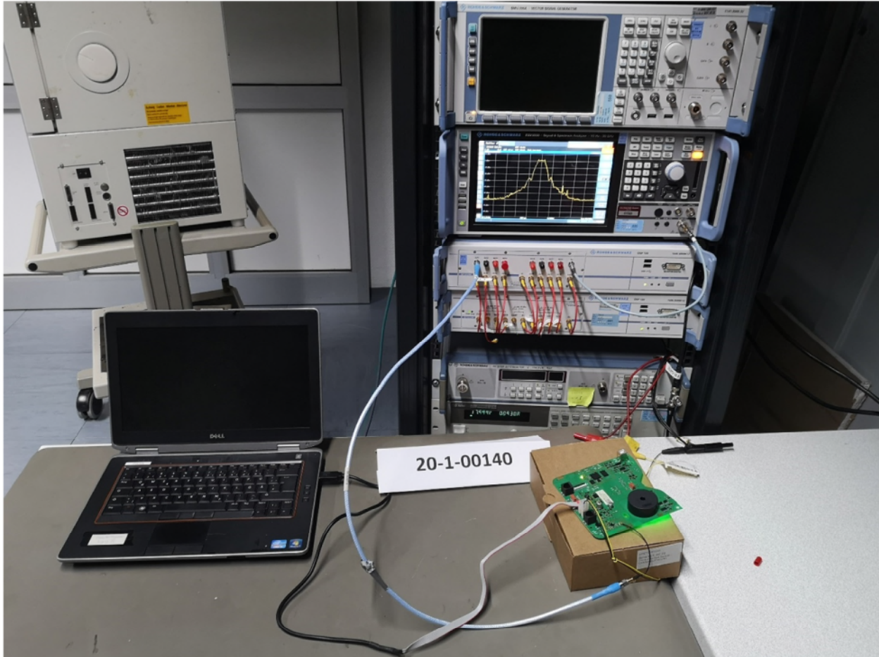
Photograph 5: EUT Setup Conducted Measurements
