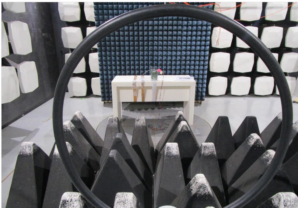
Photograph 6: H-field test setup in the semi anechoic chamber, overview
