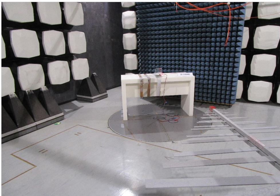
Photograph 4: EMI test setup in the semi anechoic chamber, overview
