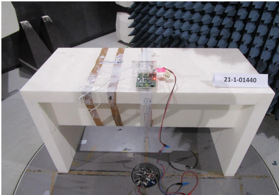
Photograph 3: EMI test setup in the semi anechoic chamber, close up view
