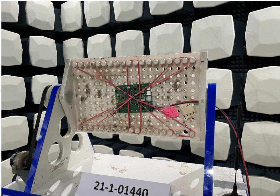
Photograph 1: EUT test setup in the fully anechoic chamber, close up view
