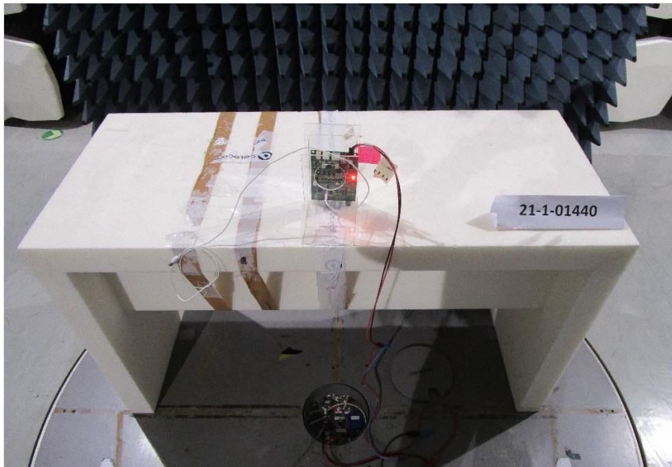
Photograph 5: H-Field test setup in the semi anechoic chamber, close up view
