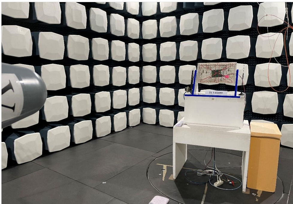
Photograph 2: EUT test setup in the fully anechoic chamber, overview
