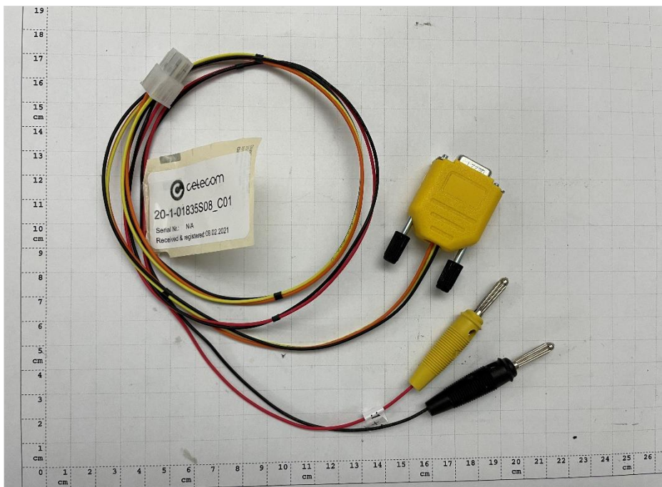
Photograph 2: CAB 01
