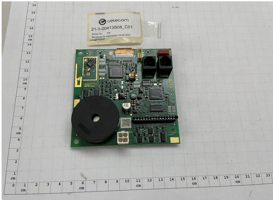
Photograph 3: EUT 2_Top side view
