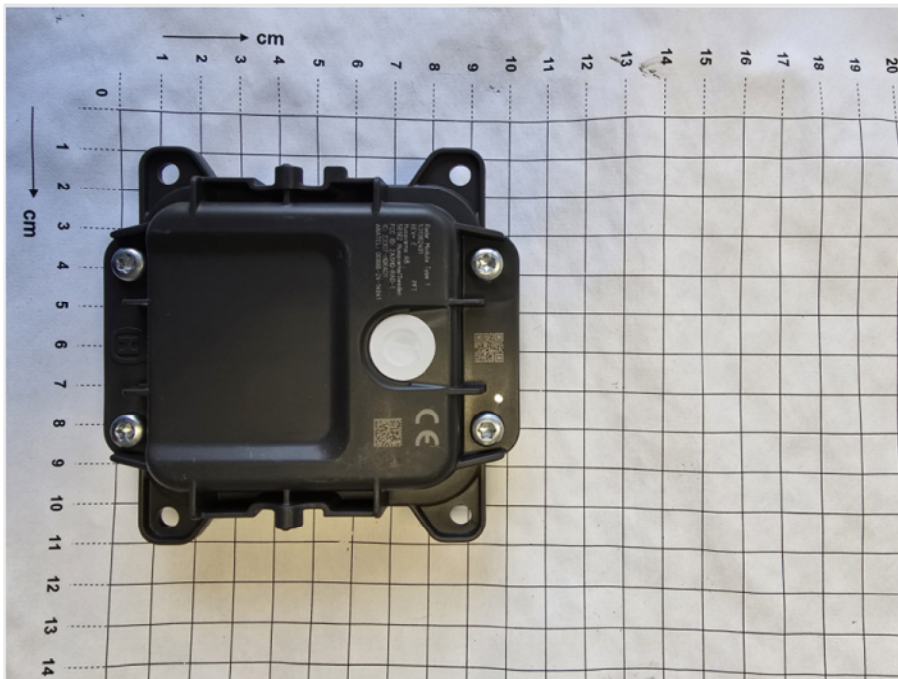
Photograph 11: EUT 3_Front side view in respect to measurements
