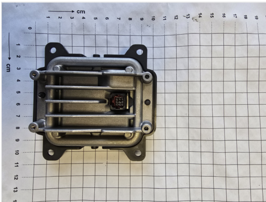
Photograph 12: EUT 3_Rear side view in respect to measurements
