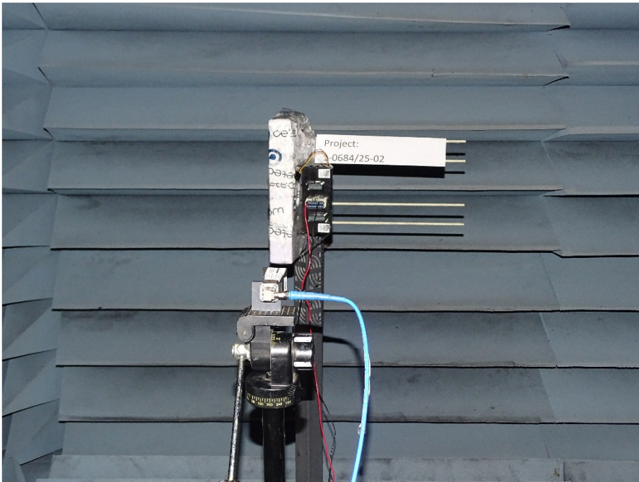
Photograph 6: EUT test setup in the fully anechoic chamber 2, overview_EUT elevation 90°
