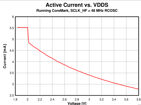
Figure 8-4. Active Mode (MCU) Current vs. Supply Voltage ( V_{\text{DD5}} ) (Running CoreMark, SCLK_HF = 48 MHz RCOSC)
