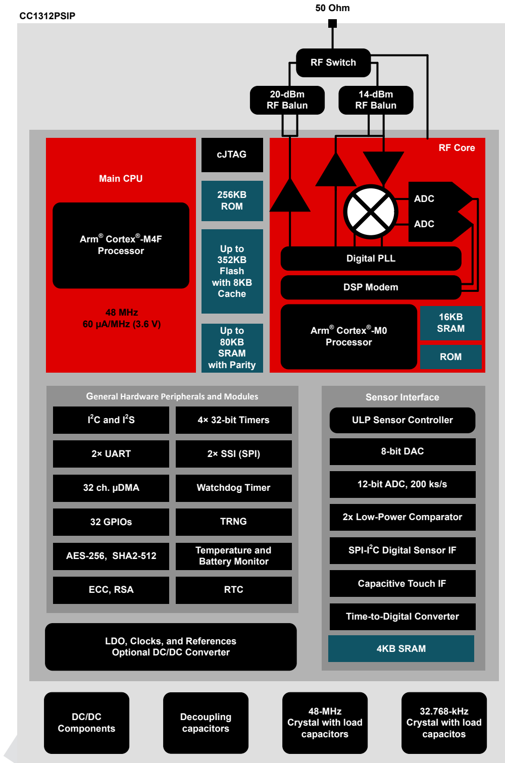
Figure 4-2. CC1312PSIP Hardware Overview
