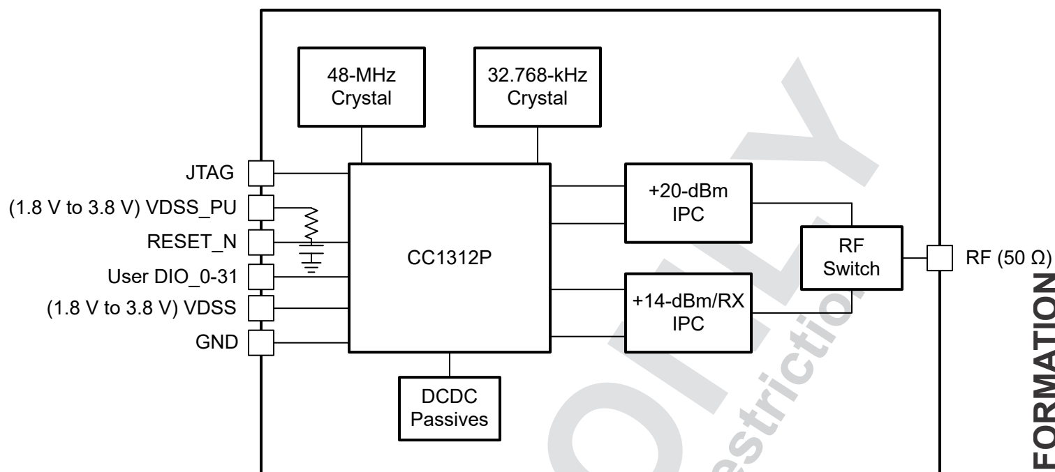
Figure 4-1. CC1312PSIP Block Diagram
