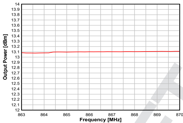
Figure 8-20. Output Power vs. Frequency (+14 dBm setting)
