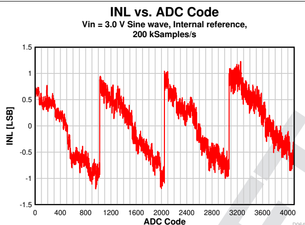
Figure 8-24. INL vs. ADC Code
