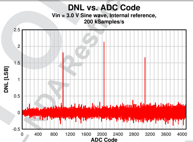
Figure 8-25. DNL vs. ADC Code
