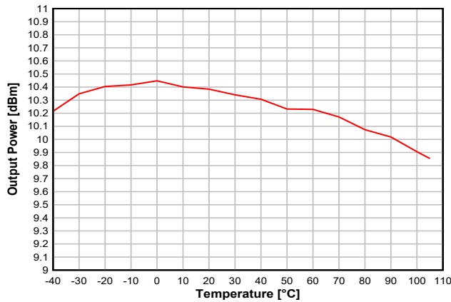
Figure 8-18. Output Power vs. Temperature (868.3 MHz, +10 dBm setting)
