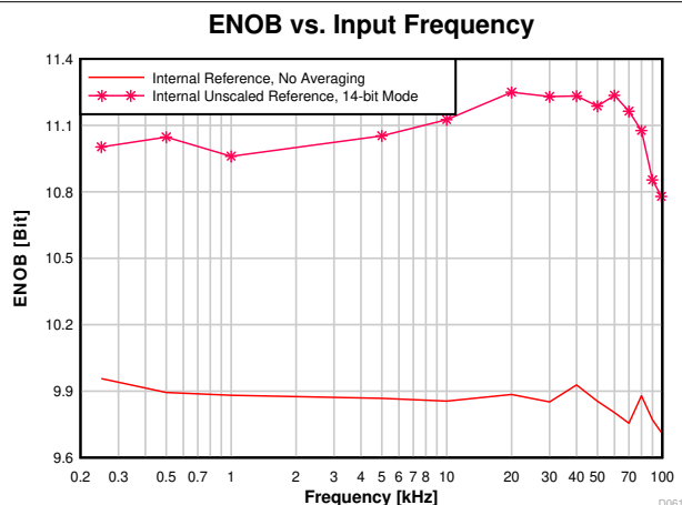
Figure 8-22. ENOB vs. Input Frequency
