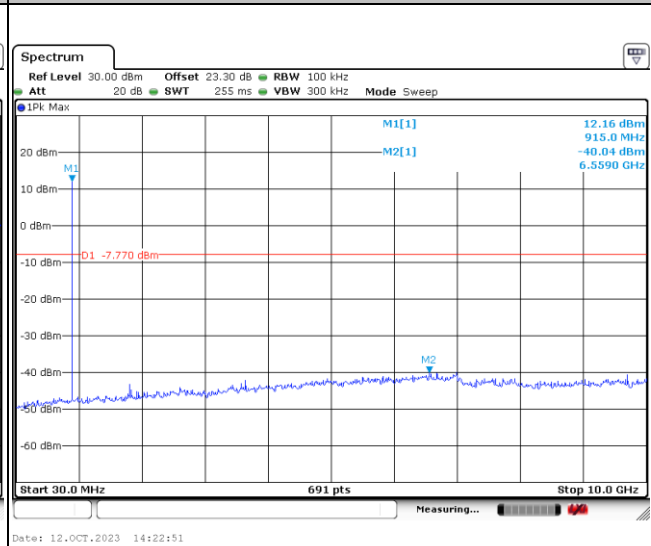
Spurious Emission 30MHz~10GHz Plot
