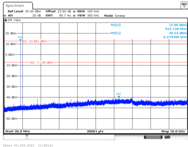
CSE Plot on Ch 65 between 30MHz ~ 10 GHz
