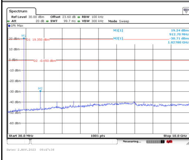
CSE Plot on Ch 01 between 30MHz ~ 10 GHz
