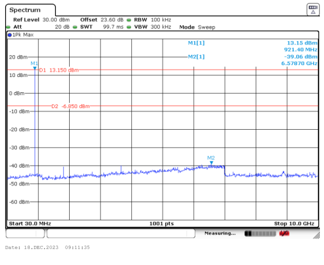
CSE Plot on Ch 50 between 30MHz ~ 10 GHz
