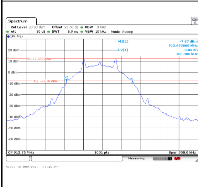
20 dB Bandwidth Plot on Channel 01
