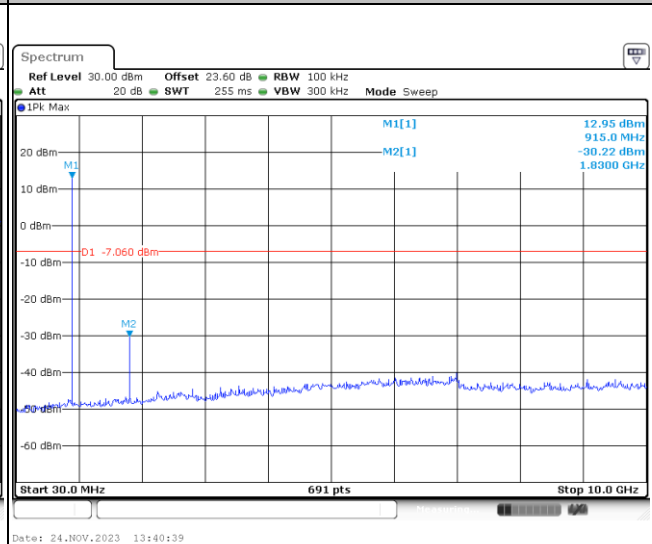
Spurious Emission 30MHz~10GHz Plot
