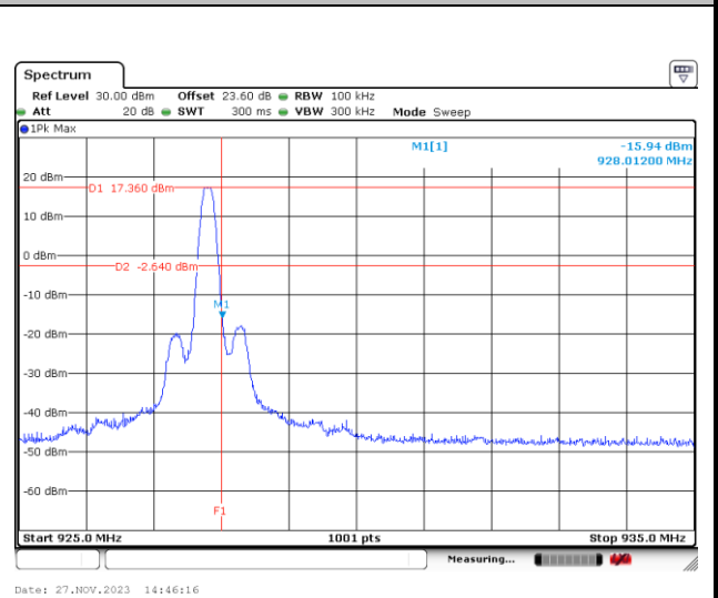
High Band Edge Plot on Channel 129
