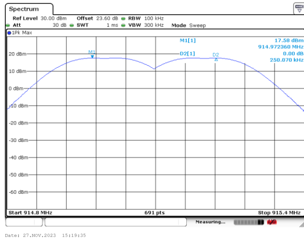
Channel Separation Plot on Channel 65 - 66
