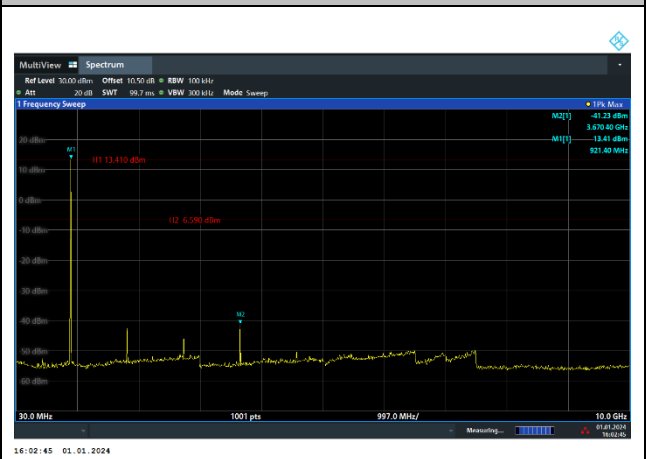
CSE Plot on Ch 50 between 30MHz ~ 10 GHz
