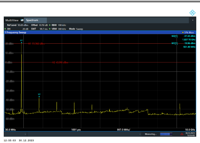
CSE Plot on Ch 50 between 30MHz ~ 10 GHz
