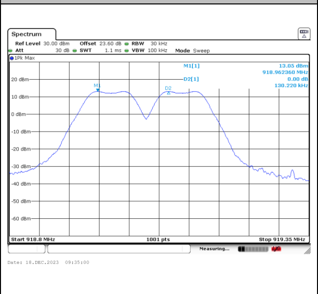
Channel Separation Plot on Channel 49 - 50
