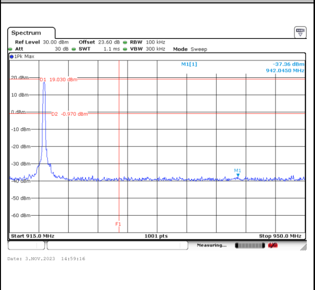
High Band Edge Plot on Channel 50
