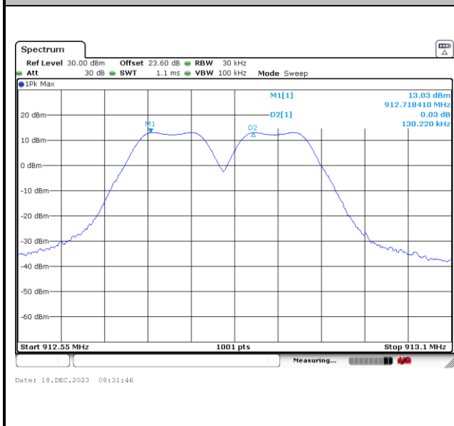
Channel Separation Plot on Channel 01 - 02
