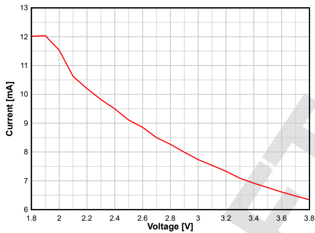
Figure 8-10. TX Current vs. Supply Voltage (VDD) (BLE 1 Mbps, 2.44 GHz, 0 dBm)
