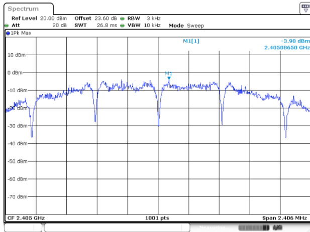
Power Density (dBm/3kHz) Plot Channel 11
