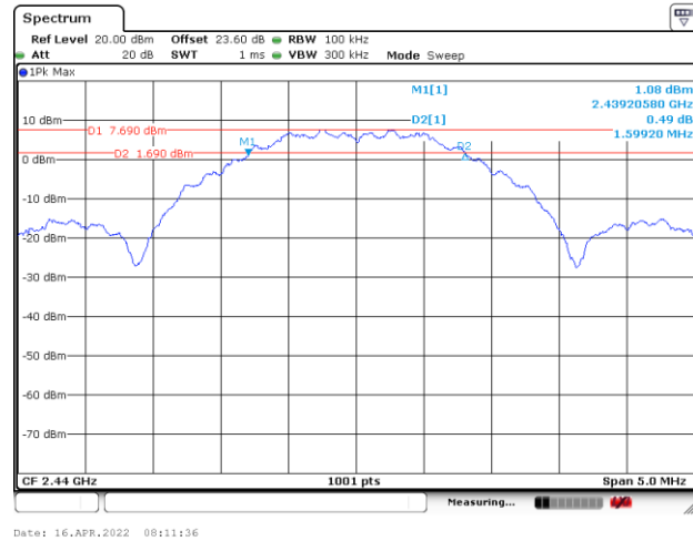
6 dB Bandwidth Plot on Channel 18
