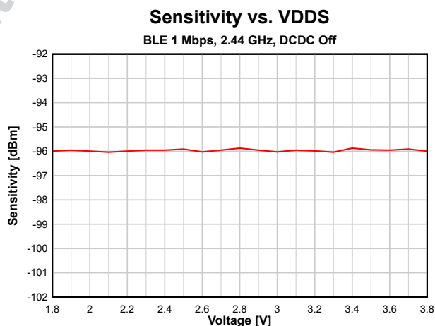
Figure 8-15. Sensitivity vs. Supply Voltage (VDD) (BLE 1 Mbps, 2.44 GHz, DCDC Off)
