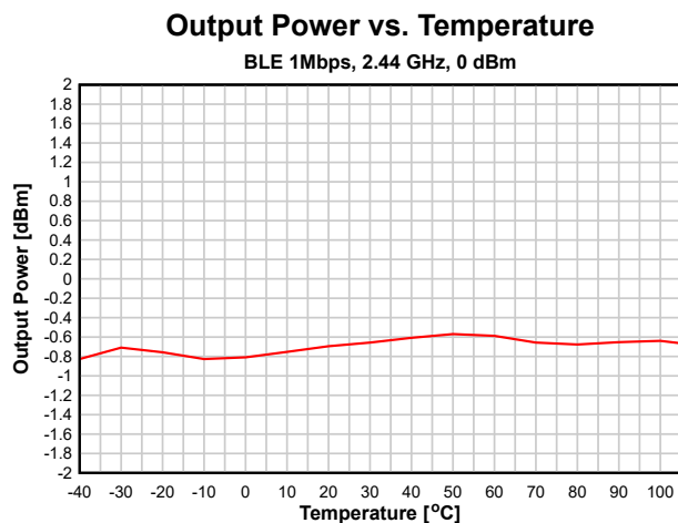
Figure 8-17. Output Power vs. Temperature (BLE 1 Mbps, 2.44 GHz)
