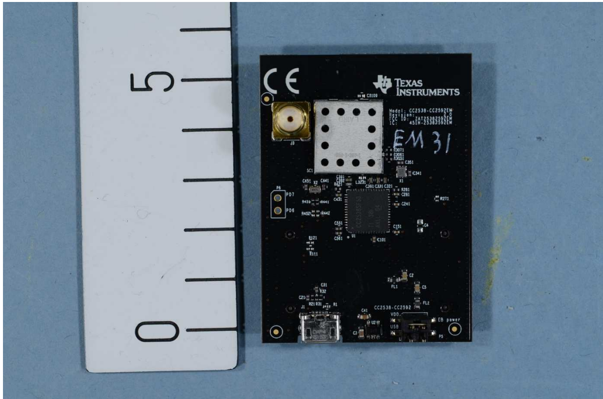
CC2538-CC2592EM – PCB component side
