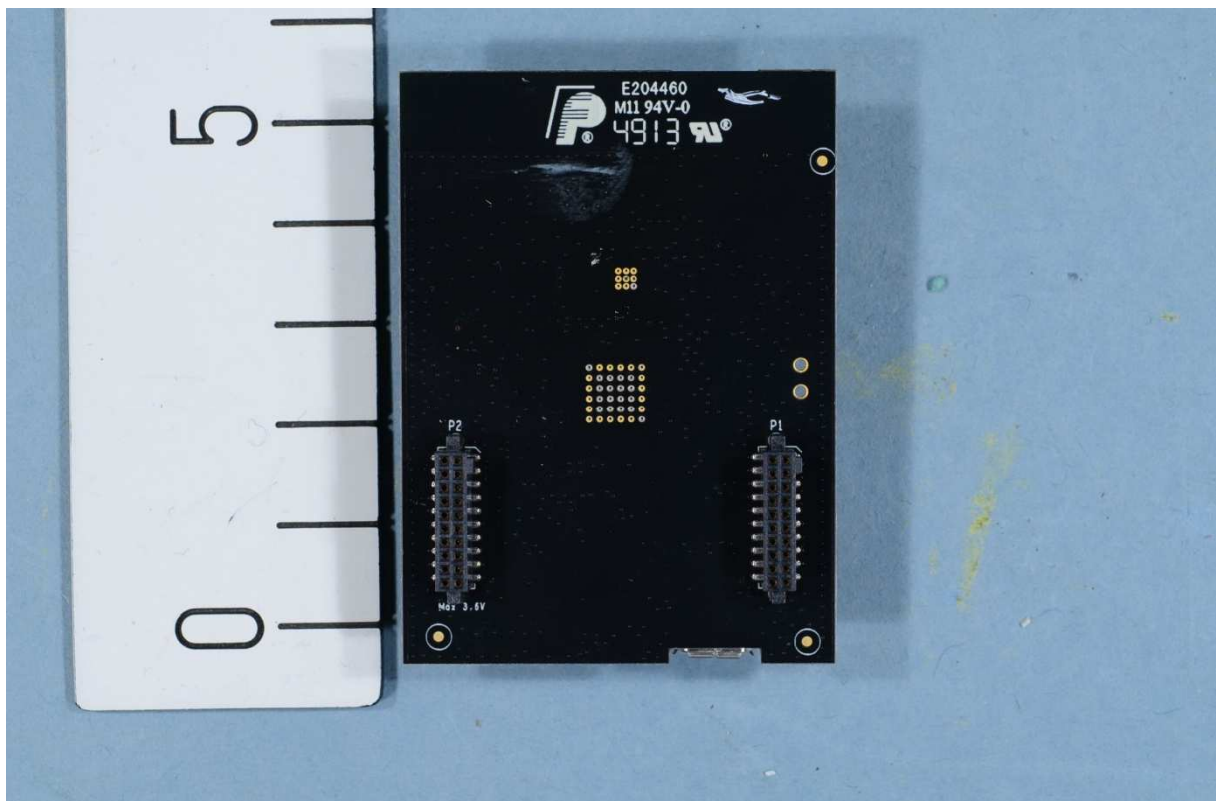
CC2538-CC2592EM – rear side
