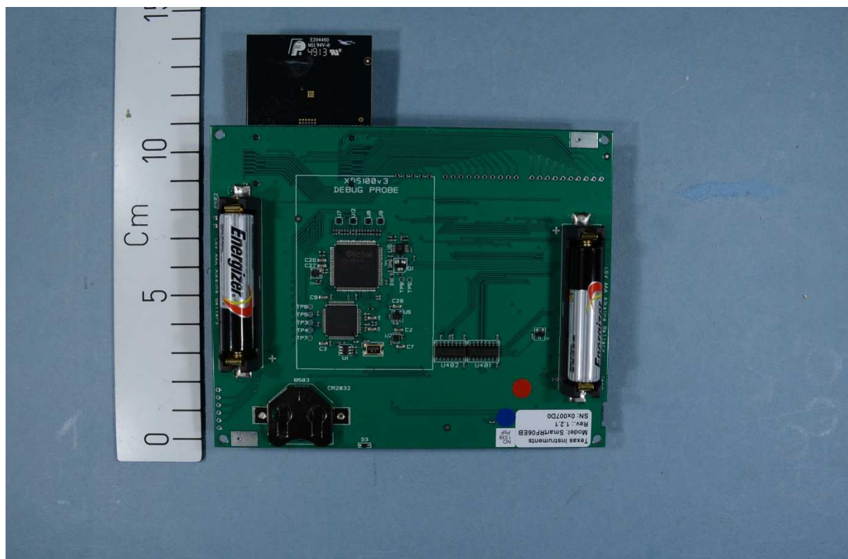
Evaluation board SmartRF06EB-rear side with 2xAAA batteries
