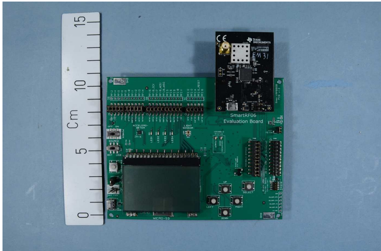
CC2538-CC2592EM with evaluation board SmartRF06EB
