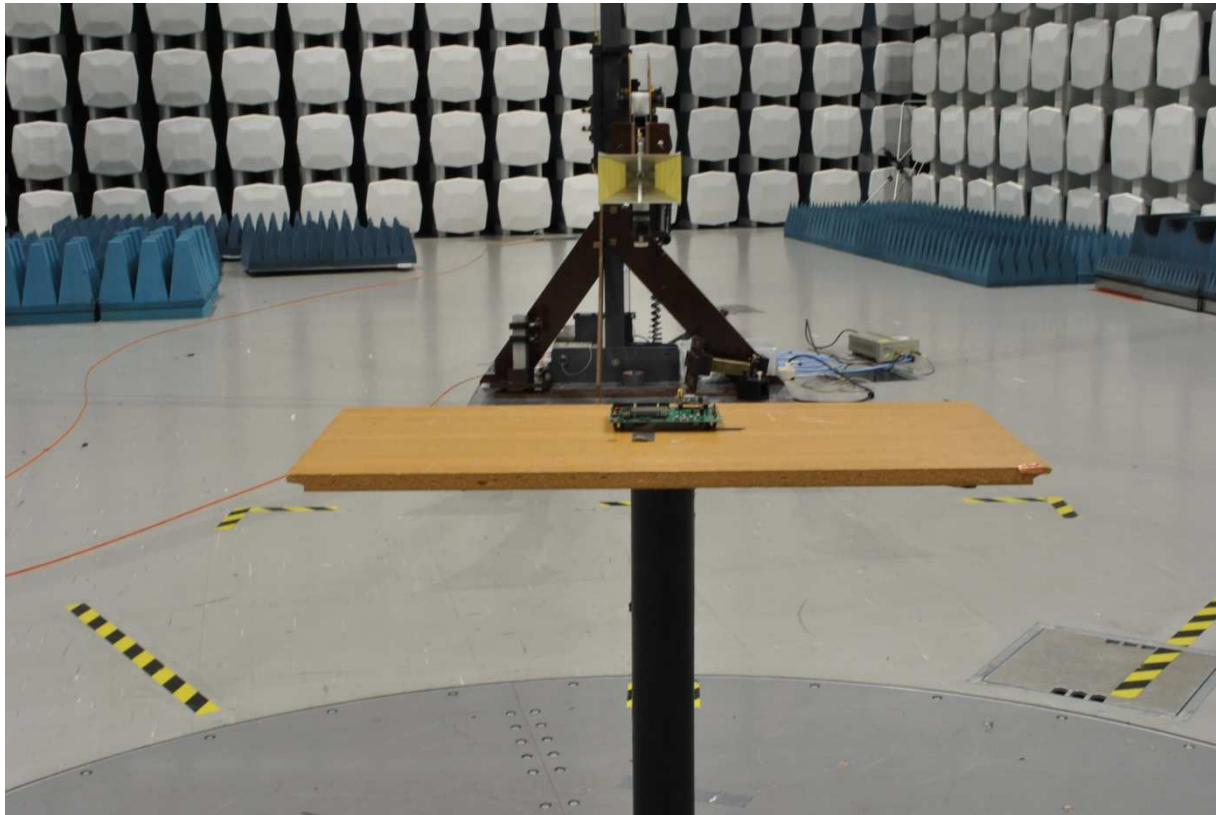
Radiated emissions 1 – 25 GHz
