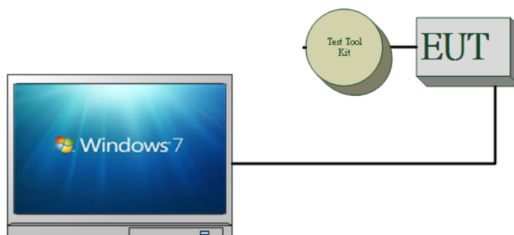
Fig. 2-2 Configuration of Conducted Emission Tested System
