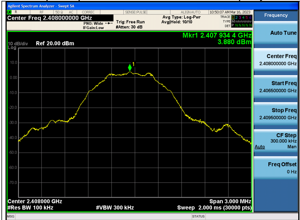
Test_Graph_GFSK_ANT1_2408_Reference Level
