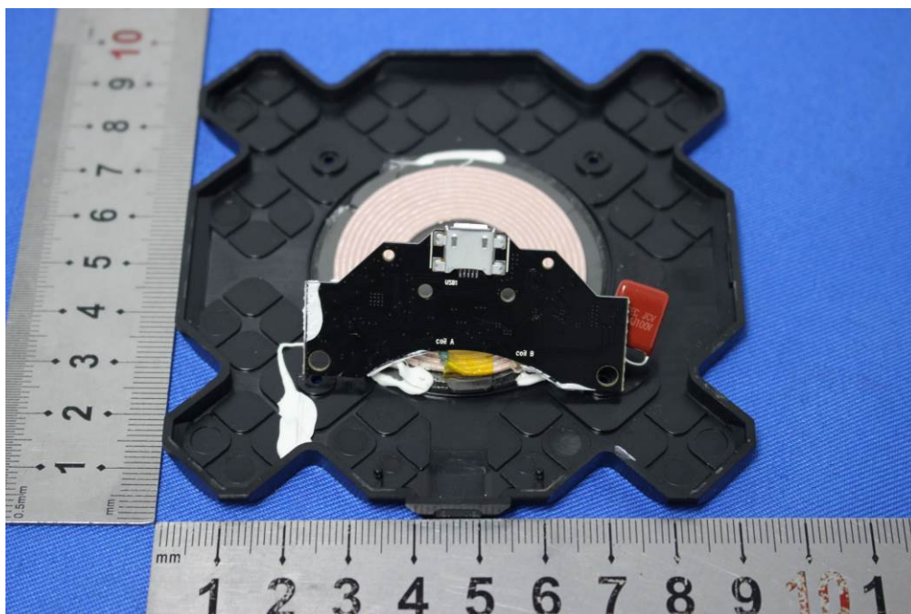
Test model No.: WD16F11 (without OVP)
