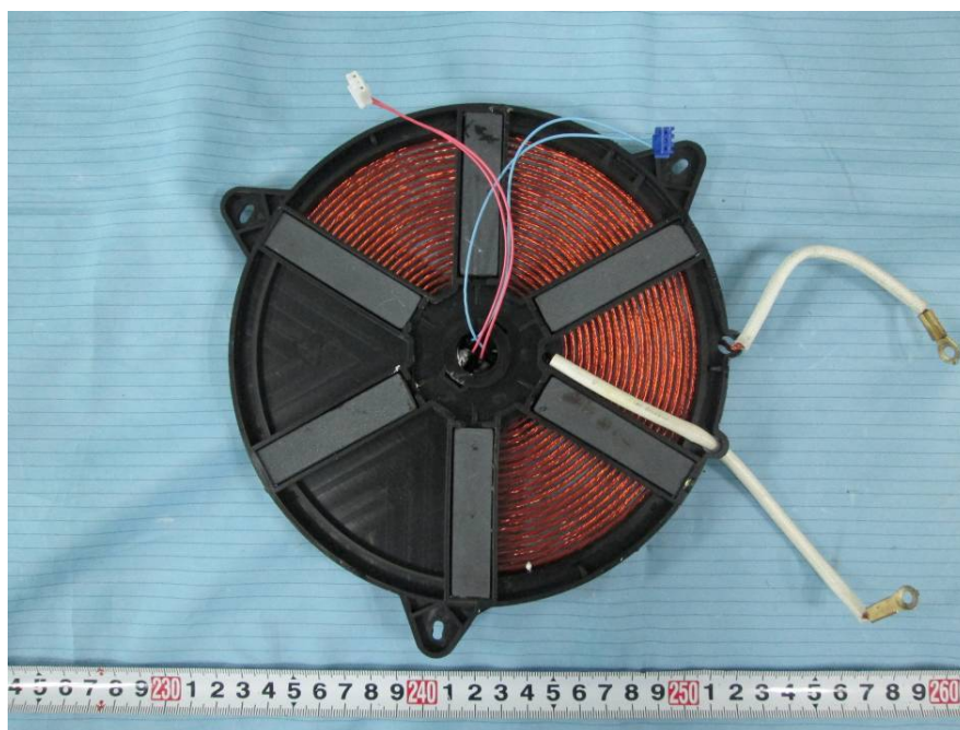
EUT – Coil Bottom View
