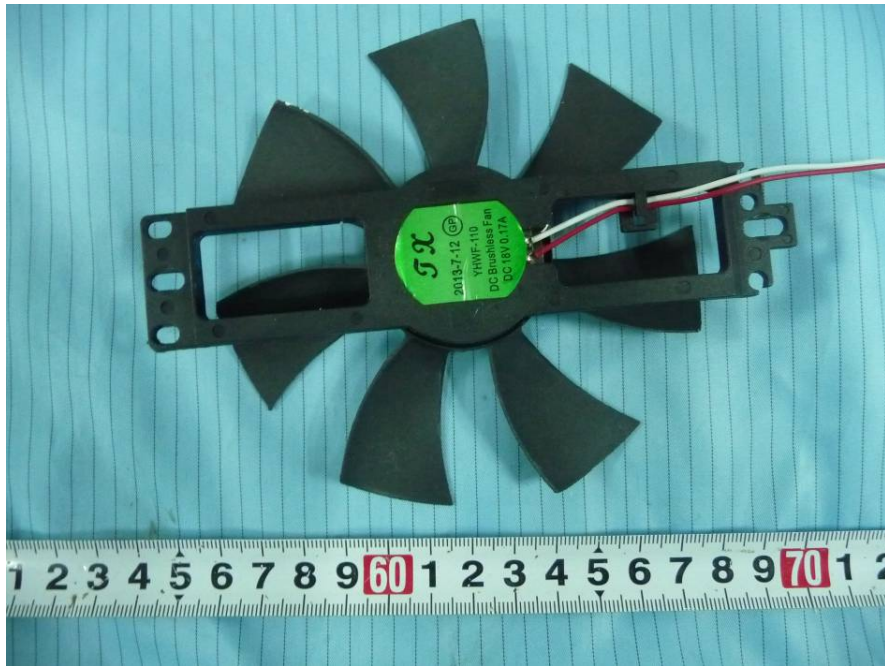
EUT-Fans Rear View
