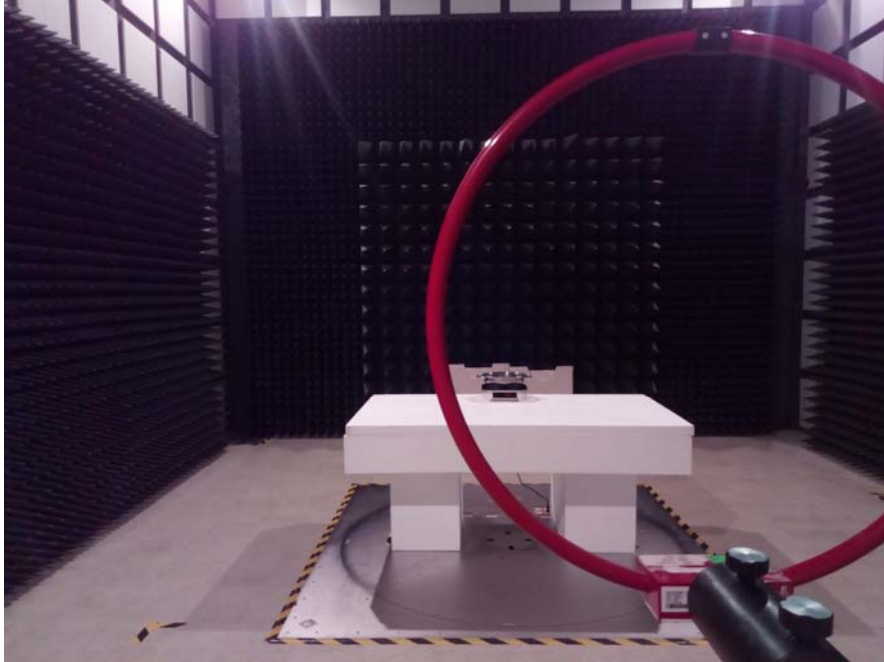
Radiated Emissions – Front View (28 kHz –30 MHz)
