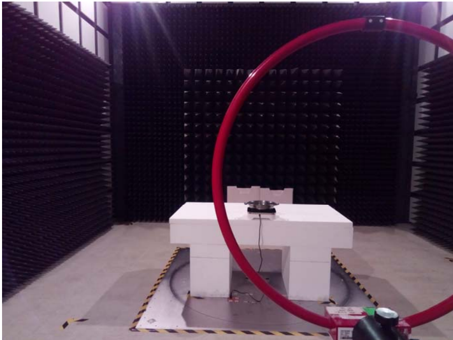
Radiated Emissions – Rear View (28 kHz –30 MHz)
