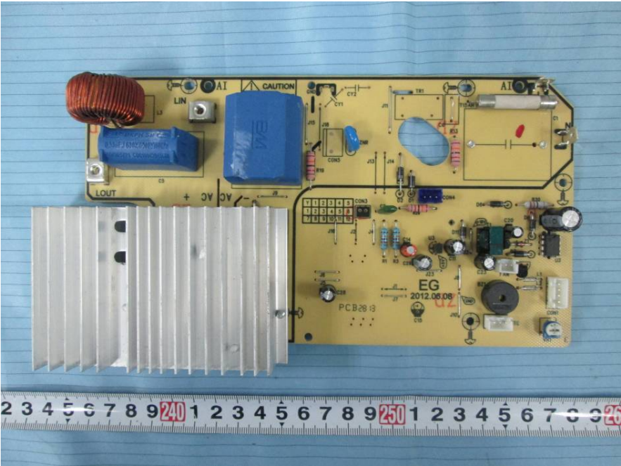
EUT – Main Board 4 Top View 1
