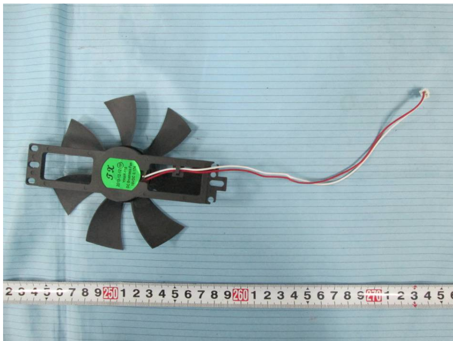
EUT –Fans 2 Bottom View
