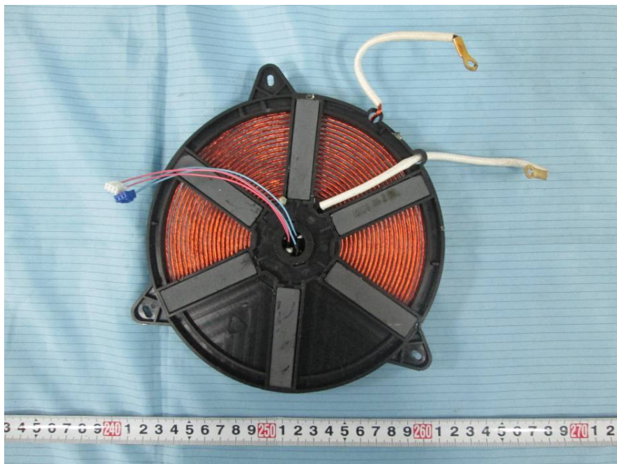
EUT – Coil 2 Bottom View
