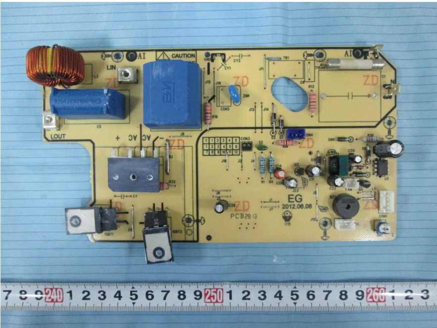
EUT – Main Board 4 Top View 2
