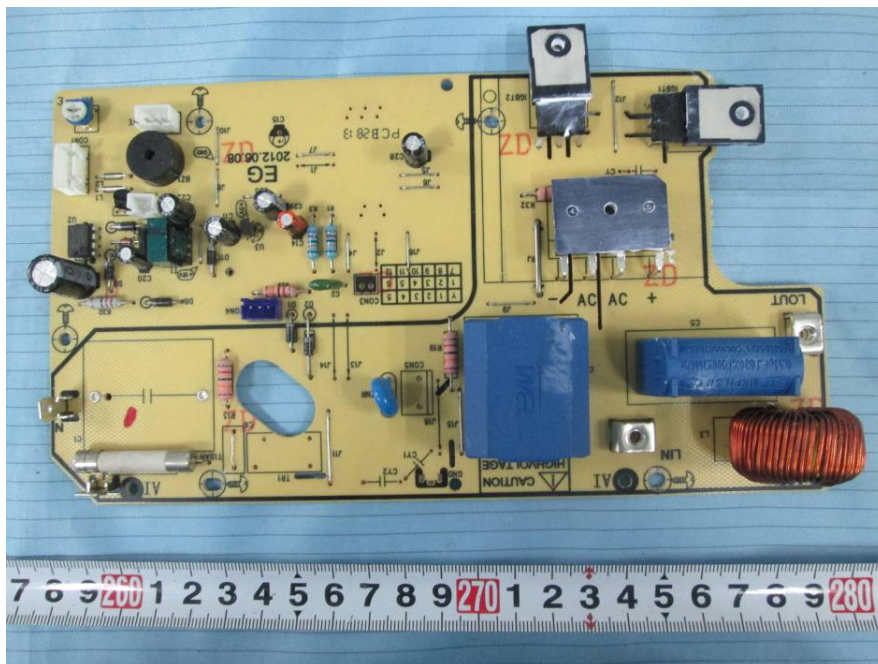
EUT – Main Board 3 Top View 2
