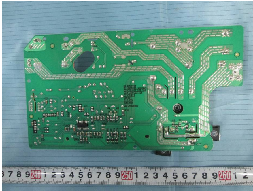
EUT – Main Board 4 Bottom View 2
