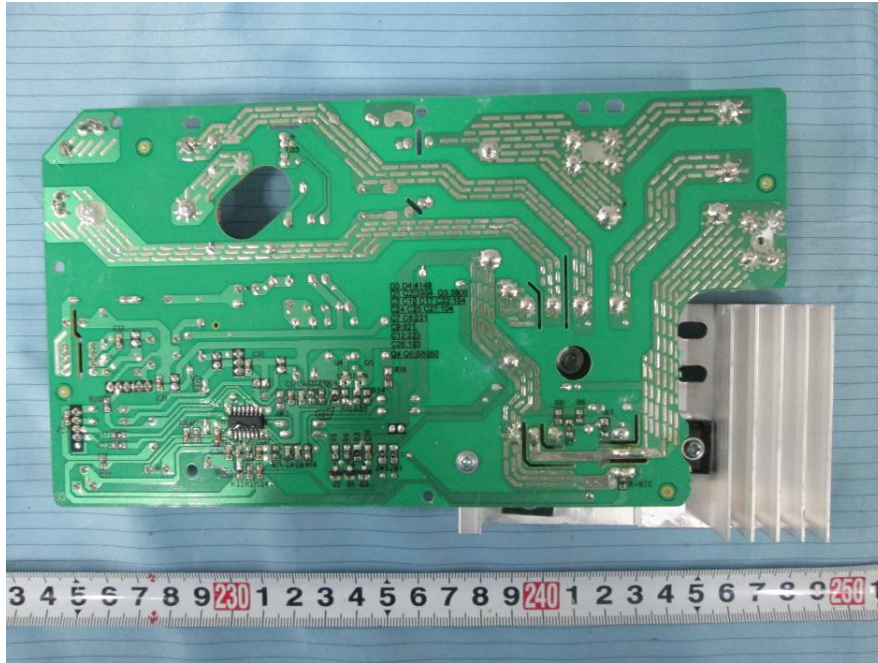
EUT – Main Board 3 Bottom View 1
