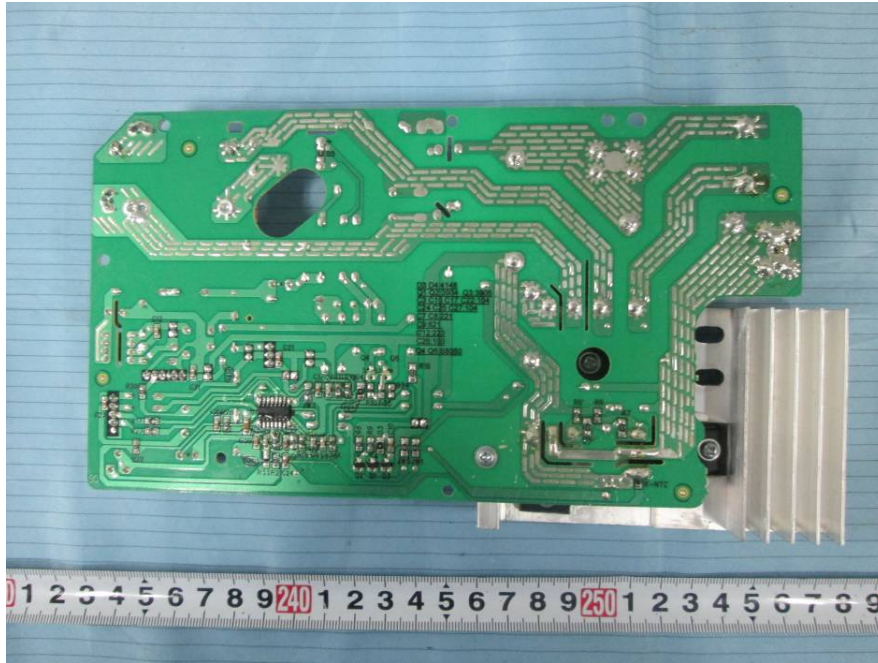
EUT – Main Board 4 Bottom View 1
