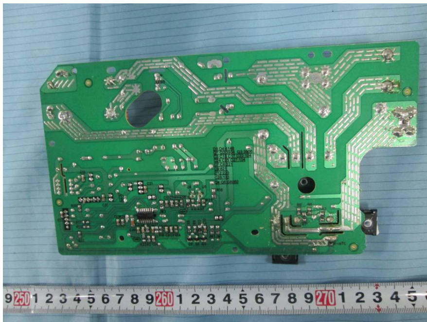
EUT – Main Board 3 Bottom View 2
