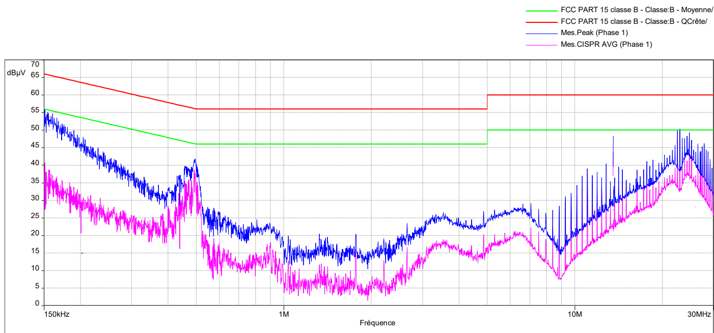
Diagram N°11 Mode POE with RF antenna Phase 120/60Hz
