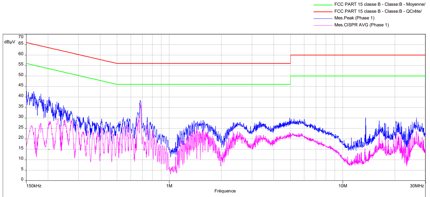
Diagram N°5 Mode DC without RF antenna Phase 240V/50Hz
