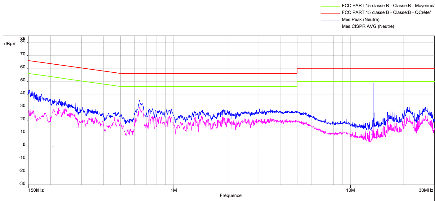
Diagram N°8 Mode DC without RF antenna Neutral 120/60Hz
