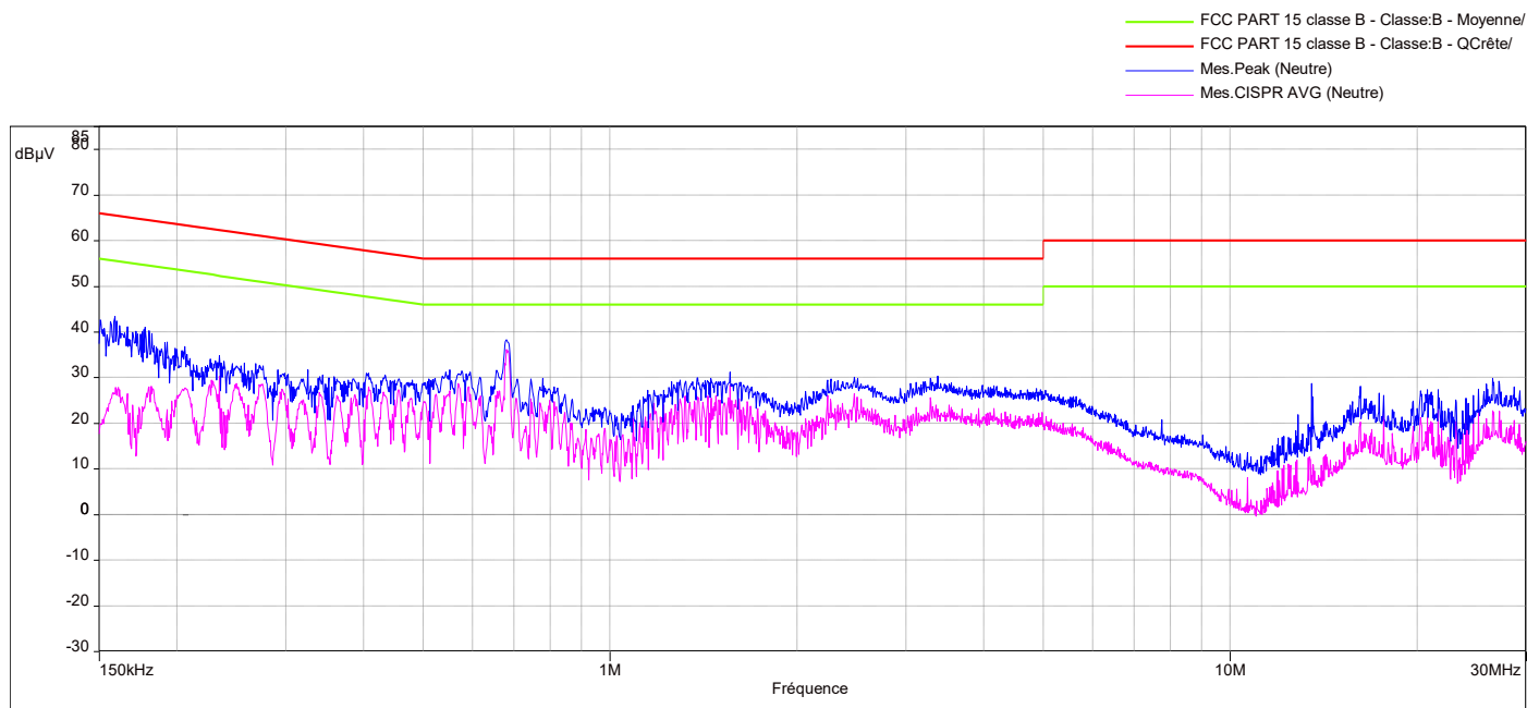
Diagram N°6 Mode DC without RF antenna Neutral 240V/50Hz
