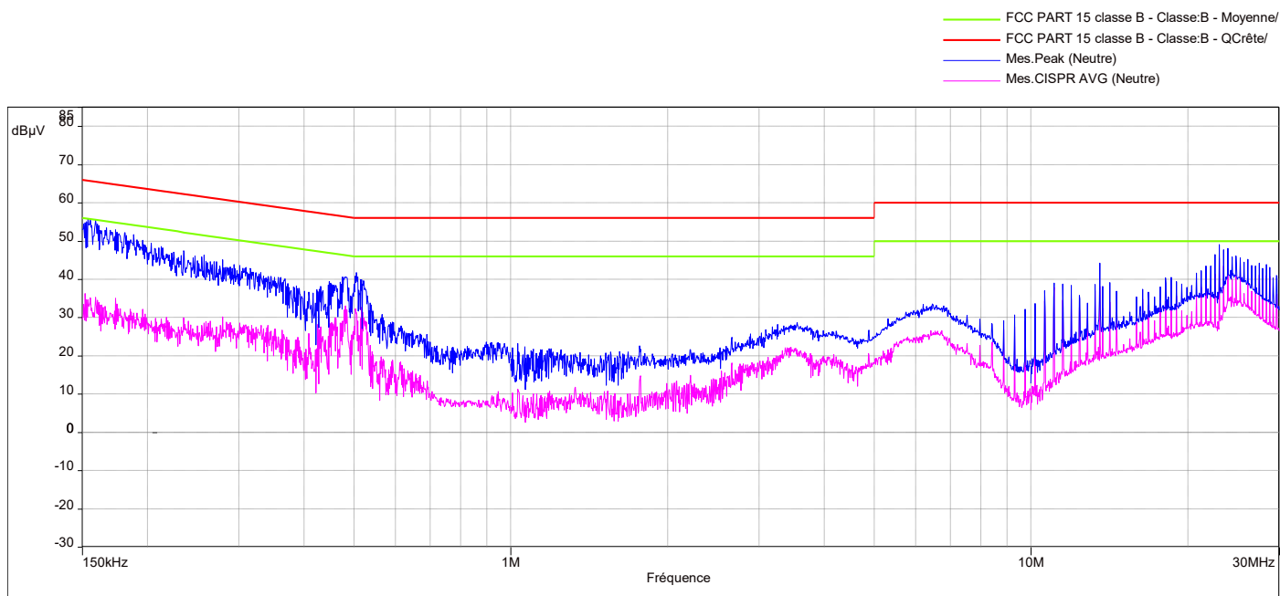
Diagram N°10 Mode POE with RF antenna Neutral 240V/50Hz
