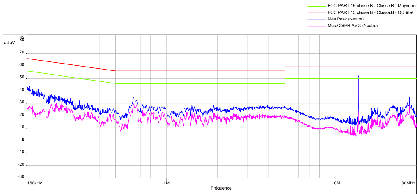
Diagram N°4 Mode DC with RF antenna Neutral 120/60Hz
