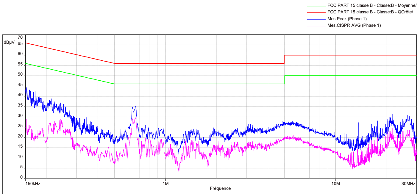
Diagram N°7 Mode DC without RF antenna Phase 120/60Hz
