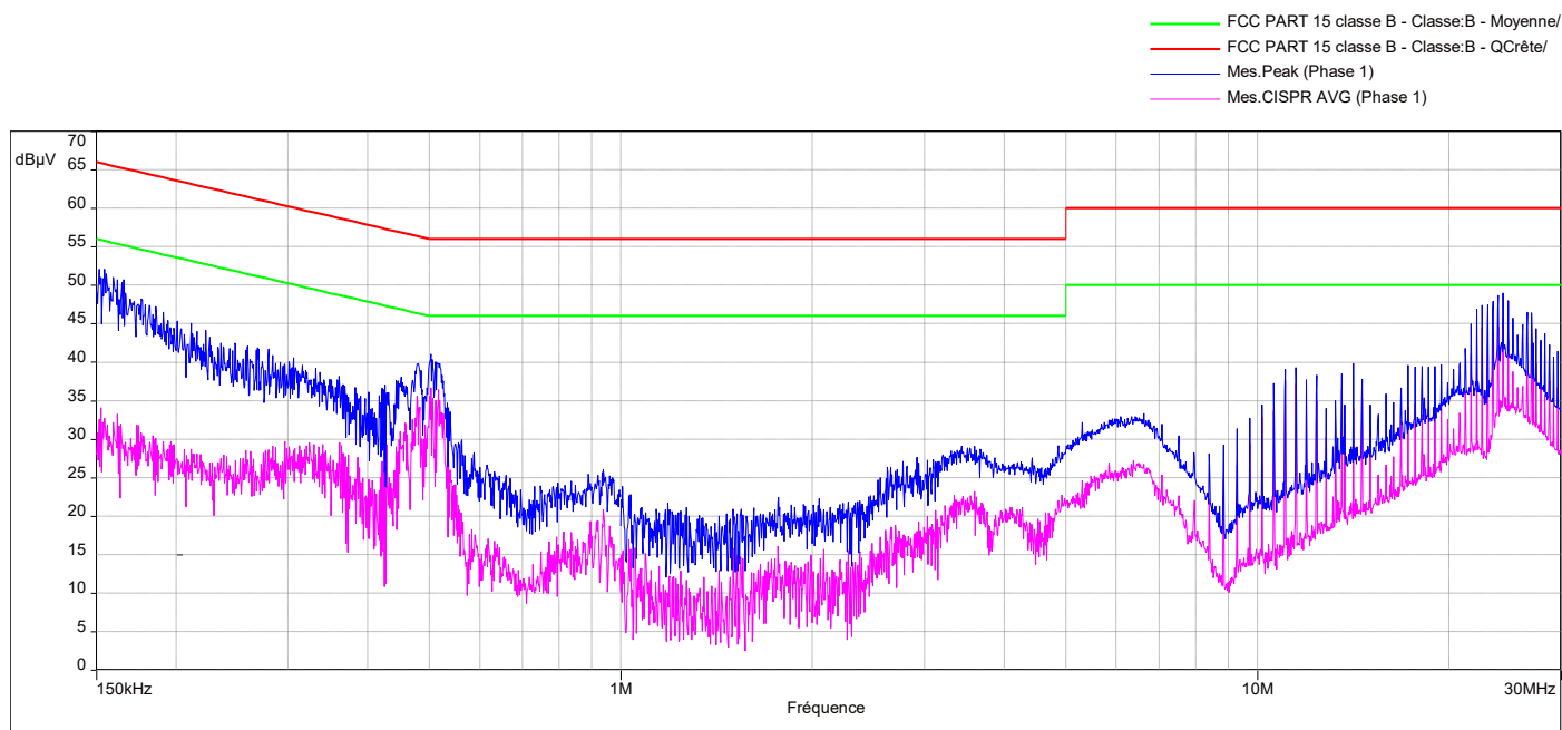
Diagram N°9 Mode POE with RF antenna Phase 240V/50Hz
